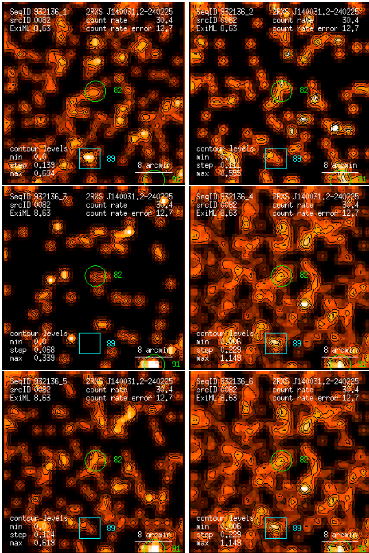
Figure 82: RASS 932136: detection 0082: band rate images, Gaussian filter: (1) PSPC channels 11 – 41, (2) 52 – 90, (3) 91 – 201, (4) 11 – 235, (5) 52 – 201, (6) 11 – 201. Broad band rates in counts/ks. Band rate contour levels in counts/ks/arcmin 2 .
