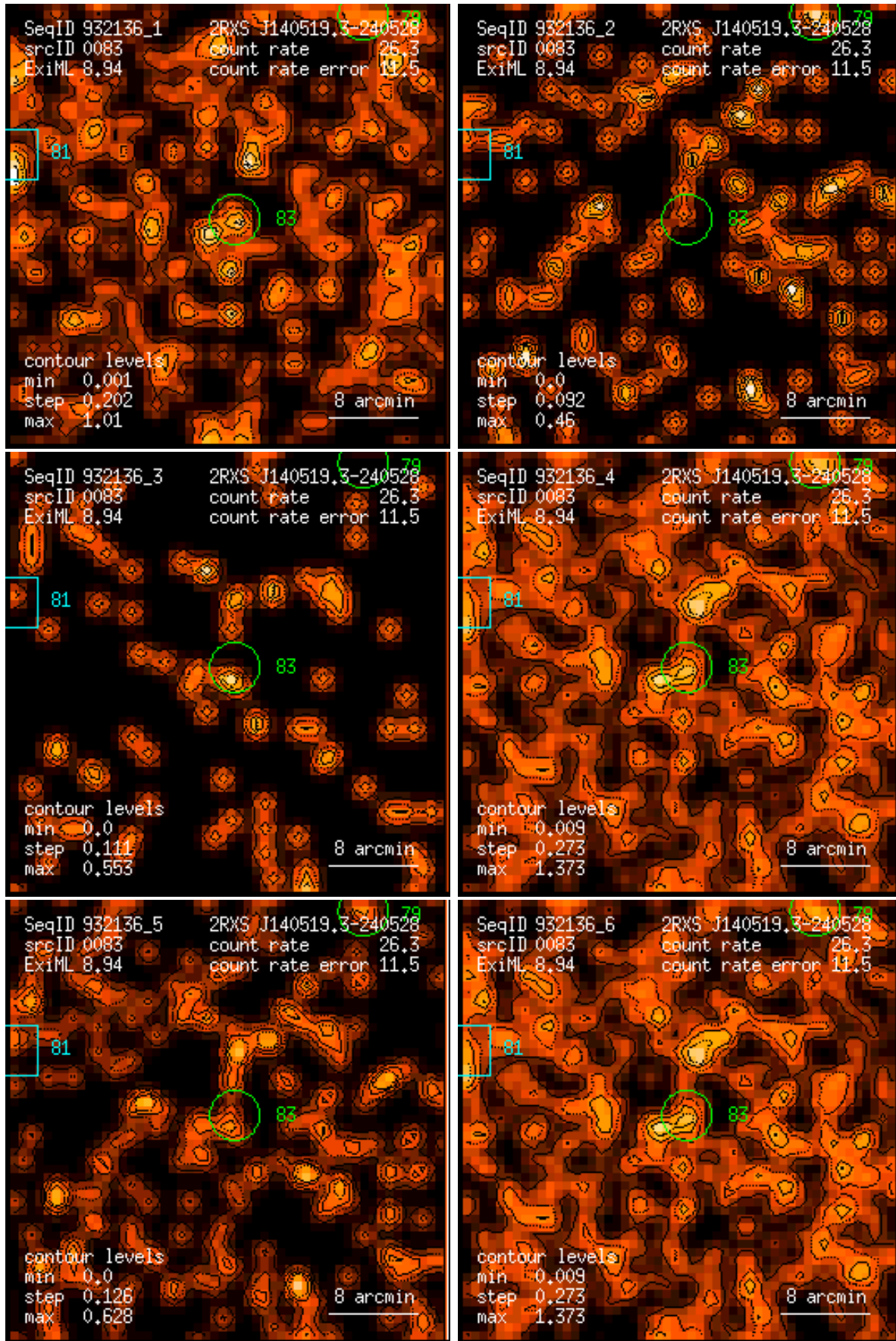
Figure 83: RASS 932136: detection 0083: band rate images, Gaussian filter: (1) PSPC channels 11 – 41, (2) 52 – 90, (3) 91 – 201, (4) 11 – 235, (5) 52 – 201, (6) 11 – 201. Broad band rates in counts/ks. Band rate contour levels in counts/ks/arcmin 2 .
