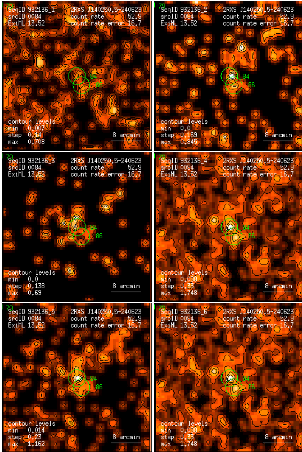
Figure 84: RASS 932136: detection 0084: band rate images, Gaussian filter: (1) PSPC channels 11 – 41, (2) 52 – 90, (3) 91 – 201, (4) 11 – 235, (5) 52 – 201, (6) 11 – 201. Broad band rates in counts/ks. Band rate contour levels in counts/ks/arcmin 2 .
