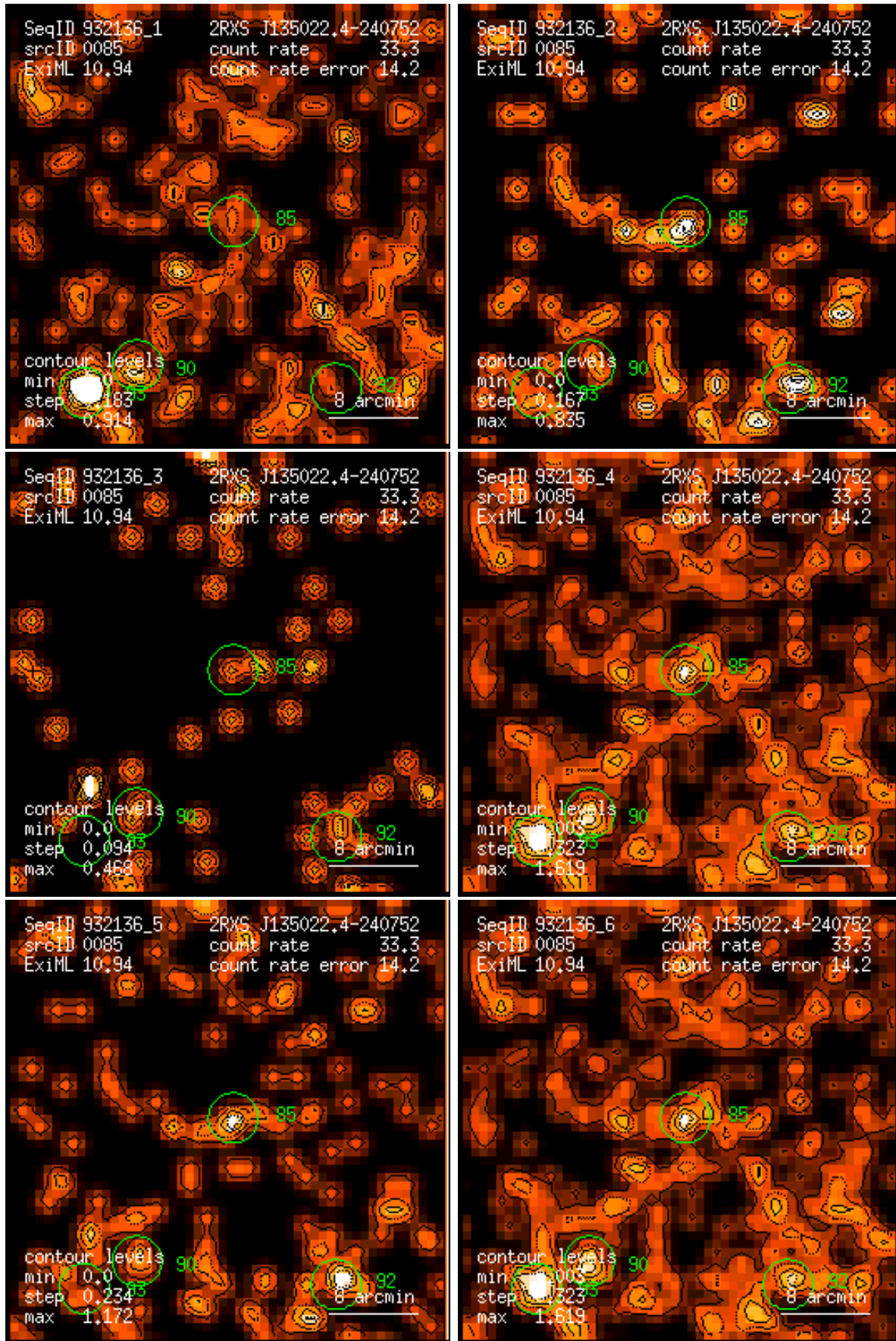
Figure 85: RASS 932136: detection 0085: band rate images, Gaussian filter: (1) PSPC channels 11 – 41, (2) 52 – 90, (3) 91 – 201, (4) 11 – 235, (5) 52 – 201, (6) 11 – 201. Broad band rates in counts/ks. Band rate contour levels in counts/ks/arcmin 2 .
