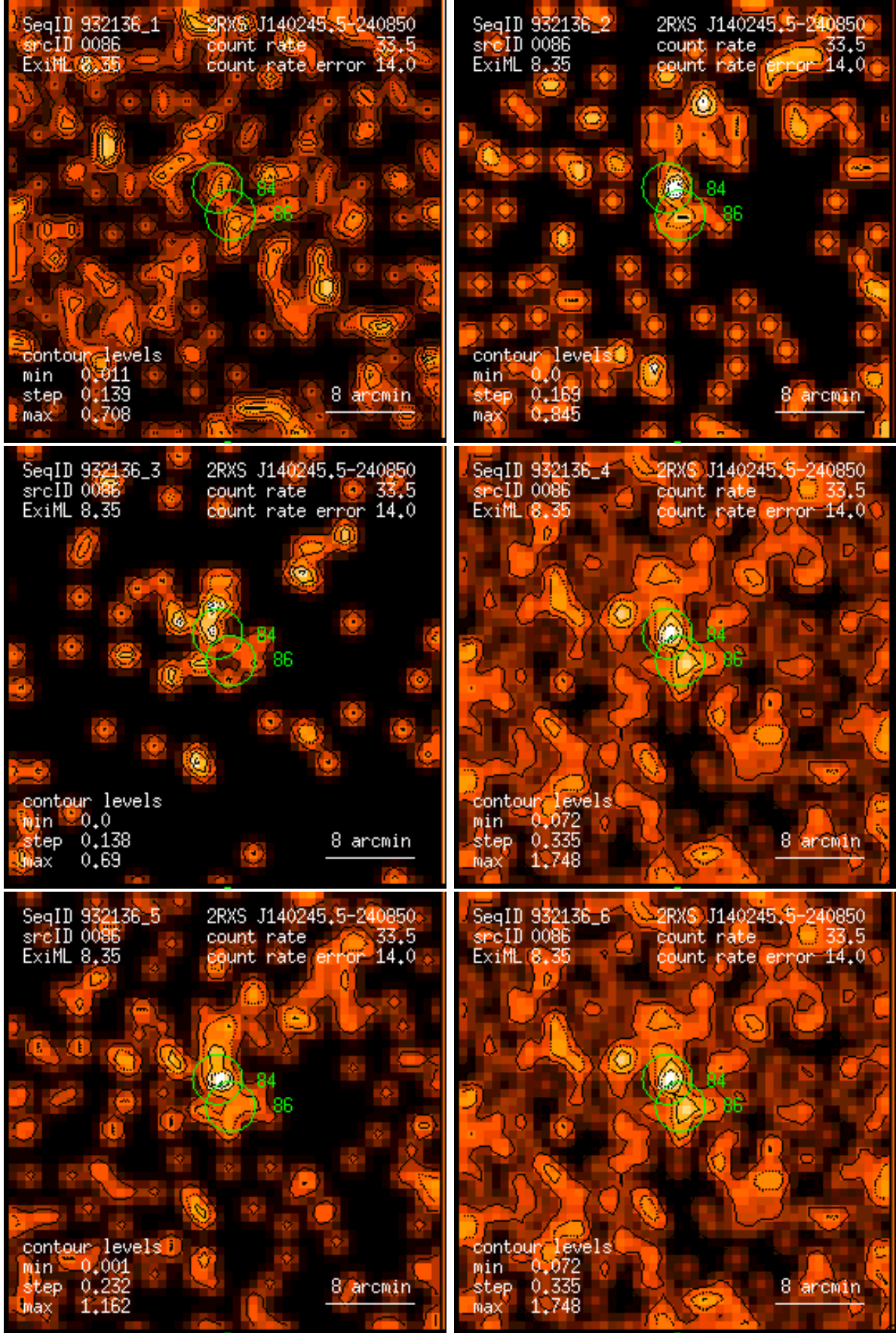
Figure 86: RASS 932136: detection 0086: band rate images, Gaussian filter: (1) PSPC channels 11 – 41, (2) 52 – 90, (3) 91 – 201, (4) 11 – 235, (5) 52 – 201, (6) 11 – 201. Broad band rates in counts/ks. Band rate contour levels in counts/ks/arcmin 2 .
