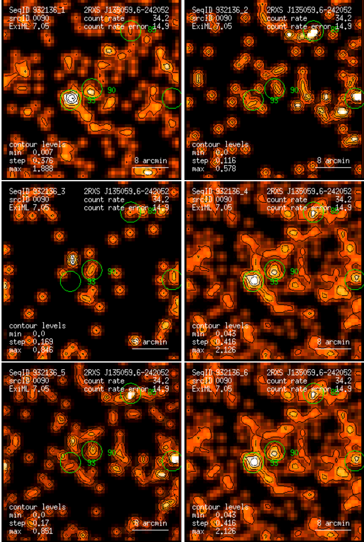
Figure 90: RASS 932136: detection 0090: band rate images, Gaussian filter: (1) PSPC channels 11 – 41, (2) 52 – 90, (3) 91 – 201, (4) 11 – 235, (5) 52 – 201, (6) 11 – 201. Broad band rates in counts/ks. Band rate contour levels in counts/ks/arcmin 2 .
