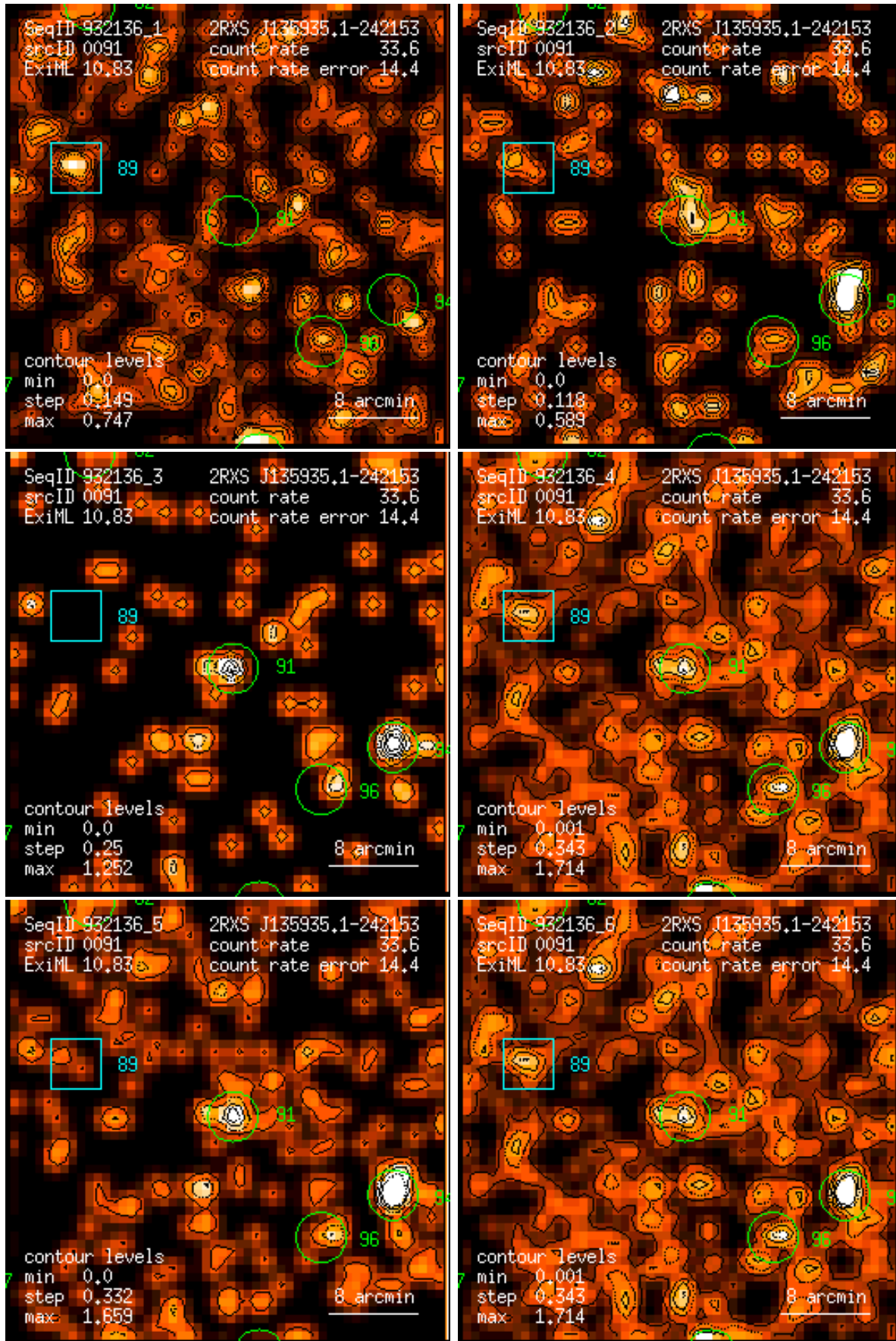
Figure 91: RASS 932136: detection 0091: band rate images, Gaussian filter: (1) PSPC channels 11 – 41, (2) 52 – 90, (3) 91 – 201, (4) 11 – 235, (5) 52 – 201, (6) 11 – 201. Broad band rates in counts/ks. Band rate contour levels in counts/ks/arcmin 2 .
