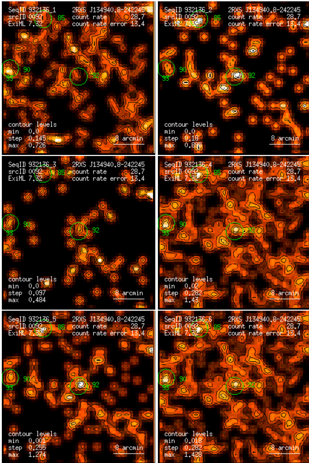
Figure 92: RASS 932136: detection 0092: band rate images, Gaussian filter: (1) PSPC channels 11 – 41, (2) 52 – 90, (3) 91 – 201, (4) 11 – 235, (5) 52 – 201, (6) 11 – 201. Broad band rates in counts/ks. Band rate contour levels in counts/ks/arcmin 2 .
