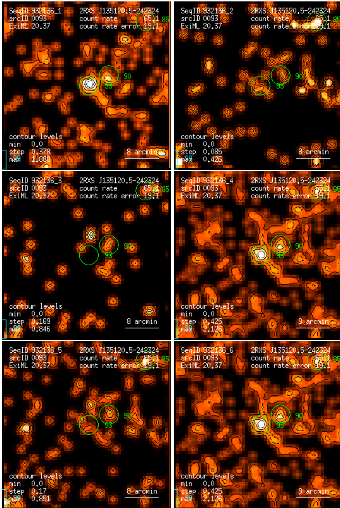
Figure 93: RASS 932136: detection 0093: band rate images, Gaussian filter: (1) PSPC channels 11 – 41, (2) 52 – 90, (3) 91 – 201, (4) 11 – 235, (5) 52 – 201, (6) 11 – 201. Broad band rates in counts/ks. Band rate contour levels in counts/ks/arcmin 2 .
