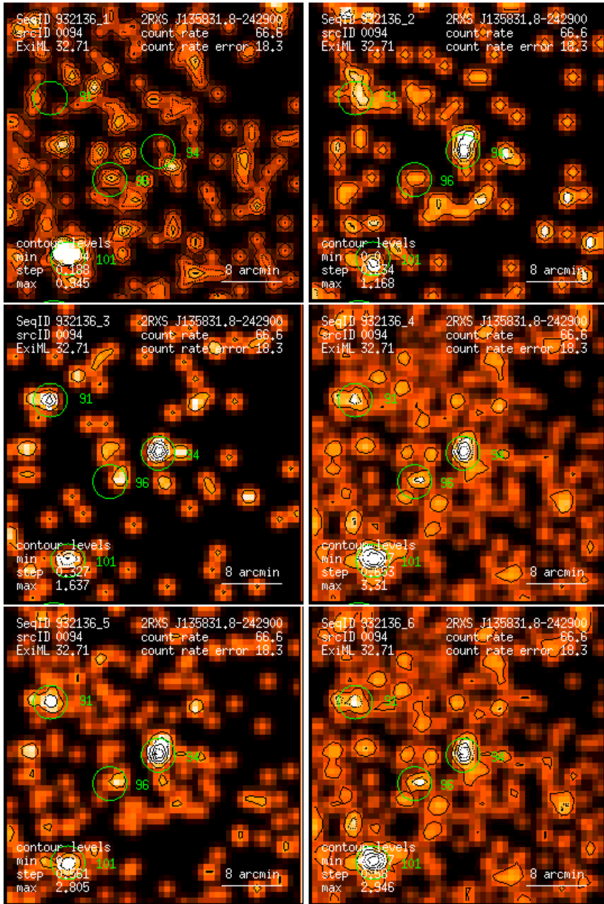
Figure 94: RASS 932136: detection 0094: band rate images, Gaussian filter: (1) PSPC channels 11 – 41, (2) 52 – 90, (3) 91 – 201, (4) 11 – 235, (5) 52 – 201, (6) 11 – 201. Broad band rates in counts/ks. Band rate contour levels in counts/ks/arcmin 2 .
