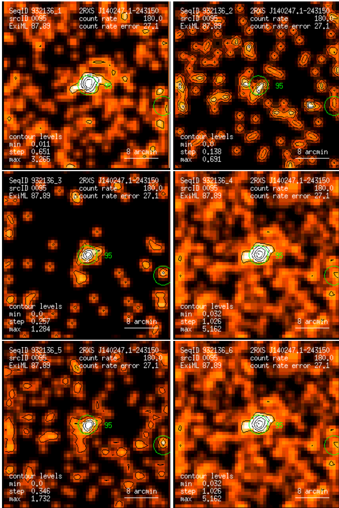
Figure 95: RASS 932136: detection 0095: band rate images, Gaussian filter: (1) PSPC channels 11 – 41, (2) 52 – 90, (3) 91 – 201, (4) 11 – 235, (5) 52 – 201, (6) 11 – 201. Broad band rates in counts/ks. Band rate contour levels in counts/ks/arcmin 2 .
