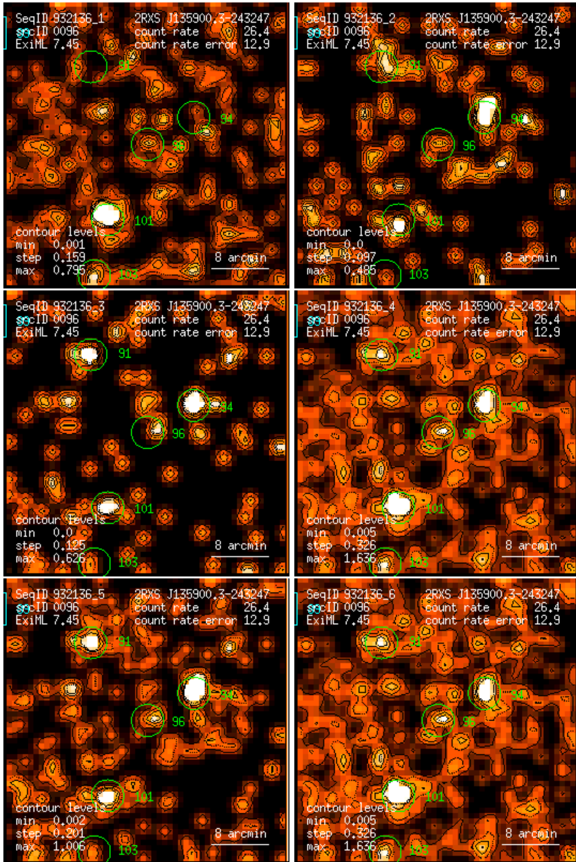
Figure 96: RASS 932136: detection 0096: band rate images, Gaussian filter: (1) PSPC channels 11 – 41, (2) 52 – 90, (3) 91 – 201, (4) 11 – 235, (5) 52 – 201, (6) 11 – 201. Broad band rates in counts/ks. Band rate contour levels in counts/ks/arcmin 2 .
