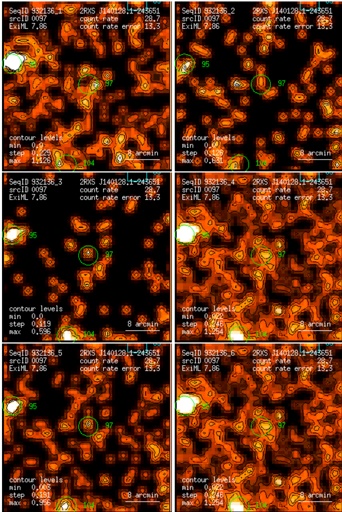
Figure 97: RASS 932136: detection 0097: band rate images, Gaussian filter: (1) PSPC channels 11 – 41, (2) 52 – 90, (3) 91 – 201, (4) 11 – 235, (5) 52 – 201, (6) 11 – 201. Broad band rates in counts/ks. Band rate contour levels in counts/ks/arcmin 2 .
