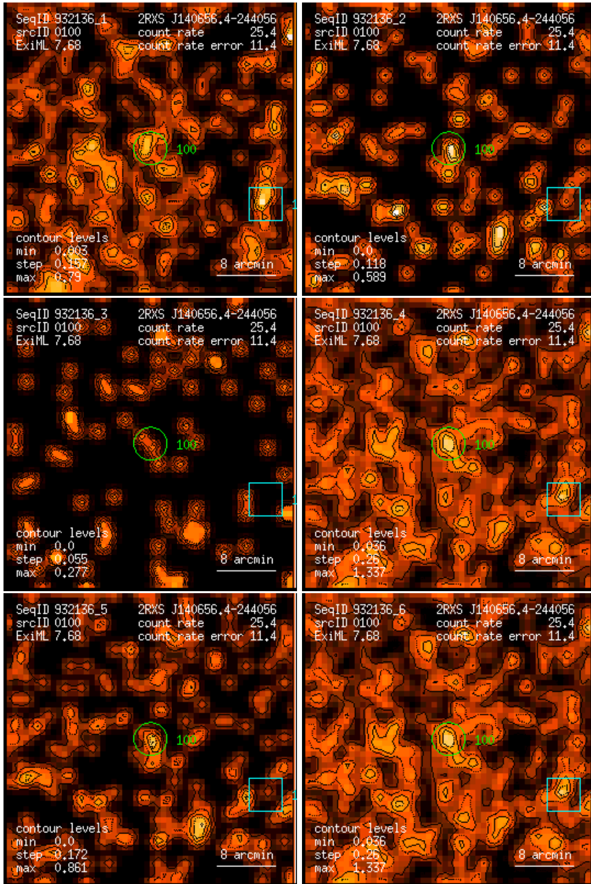
Figure 100: RASS 932136: detection 0100: band rate images, Gaussian filter: (1) PSPC channels 11 – 41, (2) 52 – 90, (3) 91 – 201, (4) 11 – 235, (5) 52 – 201, (6) 11 – 201. Broad band rates in counts/ks. Band rate contour levels in counts/ks/arcmin 2 .
