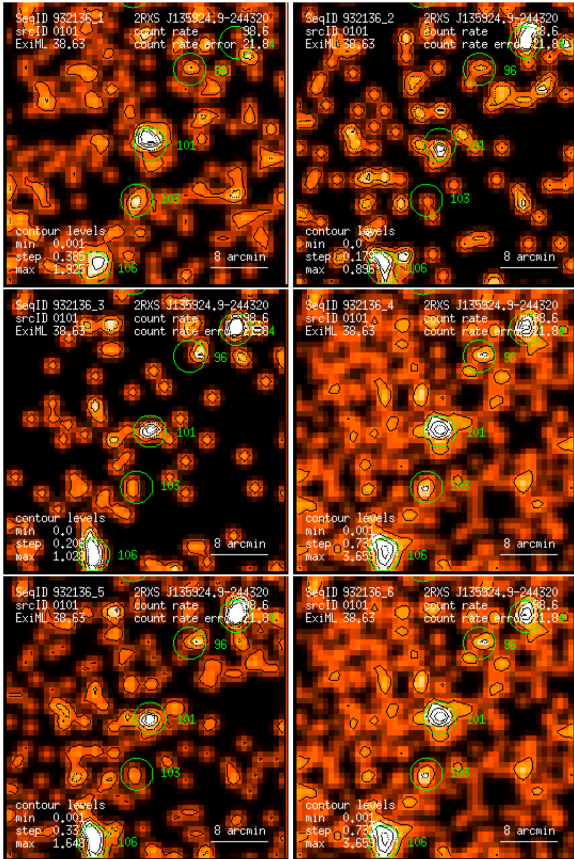
Figure 101: RASS 932136: detection 0101: band rate images, Gaussian filter: (1) PSPC channels 11 – 41, (2) 52 – 90, (3) 91 – 201, (4) 11 – 235, (5) 52 – 201, (6) 11 – 201. Broad band rates in counts/ks. Band rate contour levels in counts/ks/arcmin 2 .
