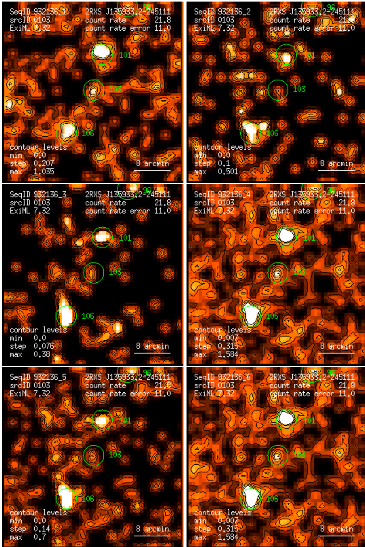
Figure 103: RASS 932136: detection 0103: band rate images, Gaussian filter: (1) PSPC channels 11 – 41, (2) 52 – 90, (3) 91 – 201, (4) 11 – 235, (5) 52 – 201, (6) 11 – 201. Broad band rates in counts/ks. Band rate contour levels in counts/ks/arcmin 2 .
