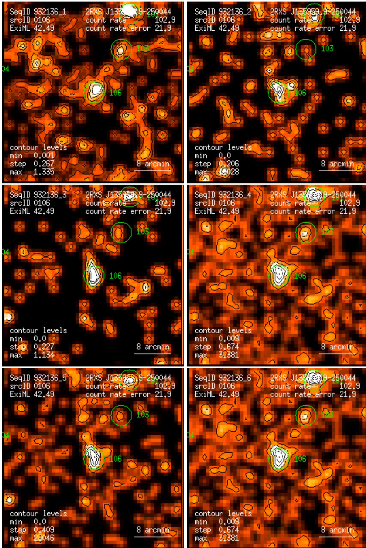
Figure 106: RASS 932136: detection 0106: band rate images, Gaussian filter: (1) PSPC channels 11 – 41, (2) 52 – 90, (3) 91 – 201, (4) 11 – 235, (5) 52 – 201, (6) 11 – 201. Broad band rates in counts/ks. Band rate contour levels in counts/ks/arcmin 2 .
