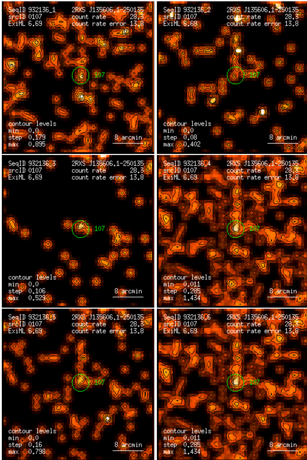
Figure 107: RASS 932136: detection 0107: band rate images, Gaussian filter: (1) PSPC channels 11 – 41, (2) 52 – 90, (3) 91 – 201, (4) 11 – 235, (5) 52 – 201, (6) 11 – 201. Broad band rates in counts/ks. Band rate contour levels in counts/ks/arcmin 2 .
