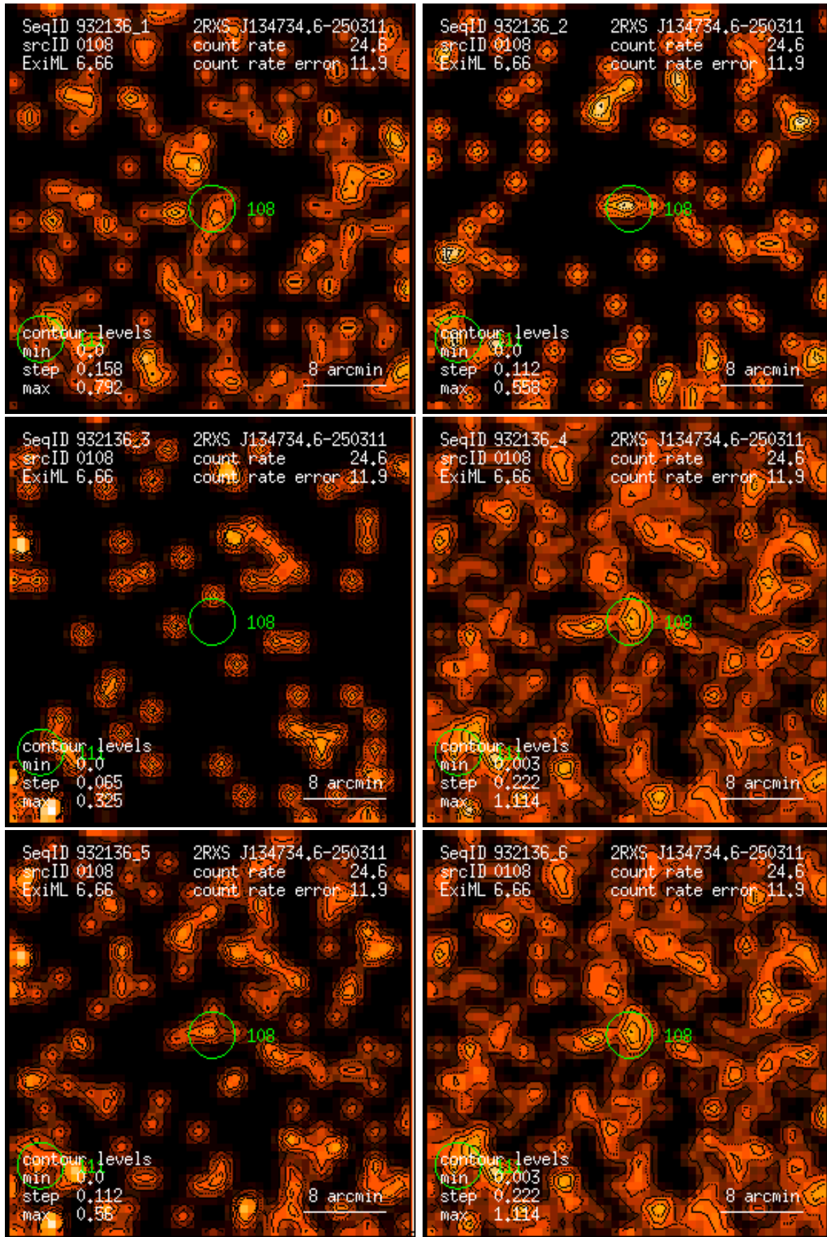
Figure 108: RASS 932136: detection 0108: band rate images, Gaussian filter: (1) PSPC channels 11 – 41, (2) 52 – 90, (3) 91 – 201, (4) 11 – 235, (5) 52 – 201, (6) 11 – 201. Broad band rates in counts/ks. Band rate contour levels in counts/ks/arcmin 2 .
