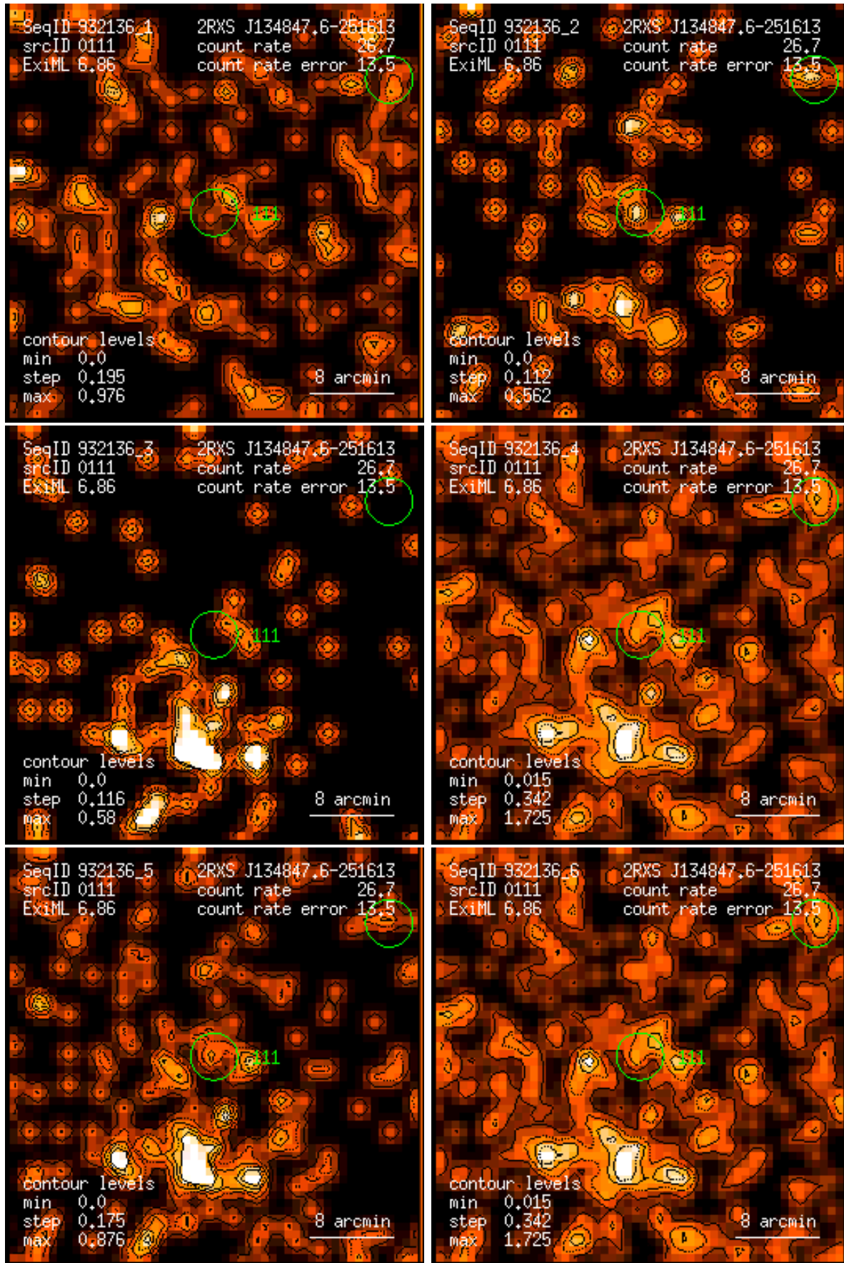
Figure 111: RASS 932136: detection 0111: band rate images, Gaussian filter: (1) PSPC channels 11 – 41, (2) 52 – 90, (3) 91 – 201, (4) 11 – 235, (5) 52 – 201, (6) 11 – 201. Broad band rates in counts/ks. Band rate contour levels in counts/ks/arcmin 2 .
