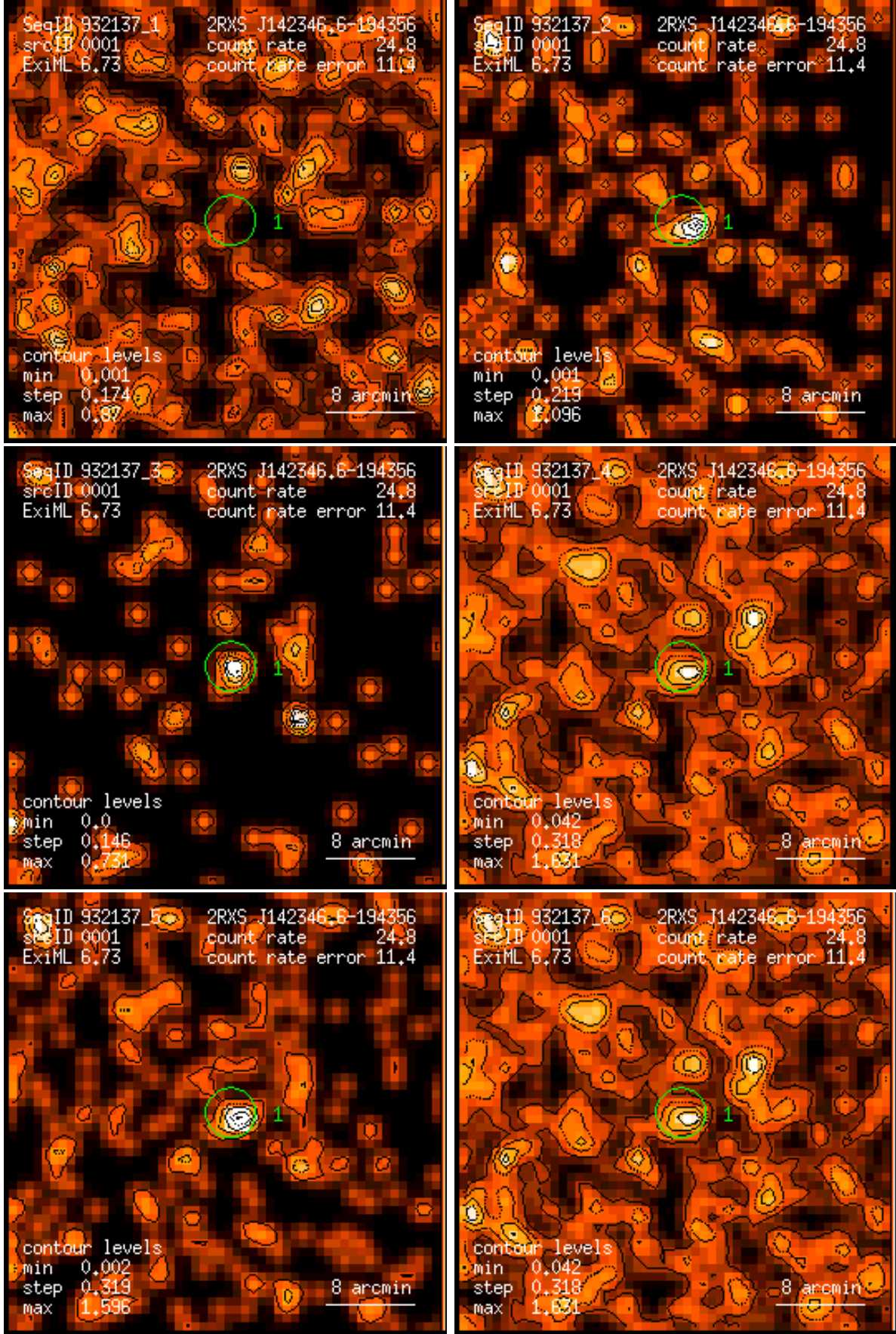
Figure 1: RASS 932137: detection 0001: band rate images, Gaussian filter: (1) PSPC channels 11 – 41, (2) 52 – 90, (3) 91 – 201, (4) 11 – 235, (5) 52 – 201, (6) 11 – 201. Broad band rates in counts/ks. Band rate contour levels in counts/ks/arcmin 2 .
