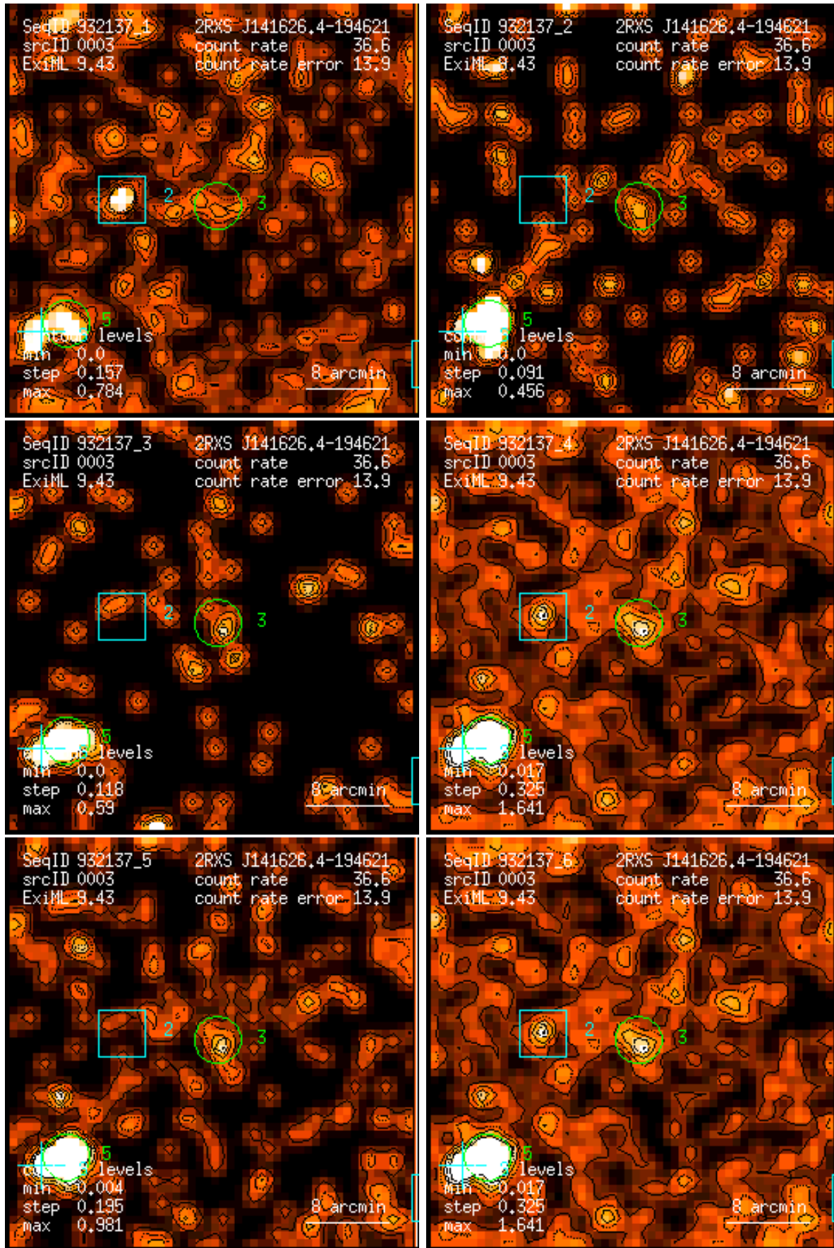
Figure 3: RASS 932137: detection 0003: band rate images, Gaussian filter: (1) PSPC channels 11 – 41, (2) 52 – 90, (3) 91 – 201, (4) 11 – 235, (5) 52 – 201, (6) 11 – 201. Broad band rates in counts/ks. Band rate contour levels in counts/ks/arcmin 2 .
