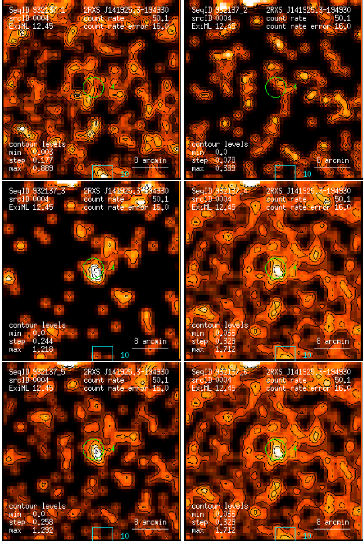
Figure 4: RASS 932137: detection 0004: band rate images, Gaussian filter: (1) PSPC channels 11 – 41, (2) 52 – 90, (3) 91 – 201, (4) 11 – 235, (5) 52 – 201, (6) 11 – 201. Broad band rates in counts/ks. Band rate contour levels in counts/ks/arcmin 2 .
