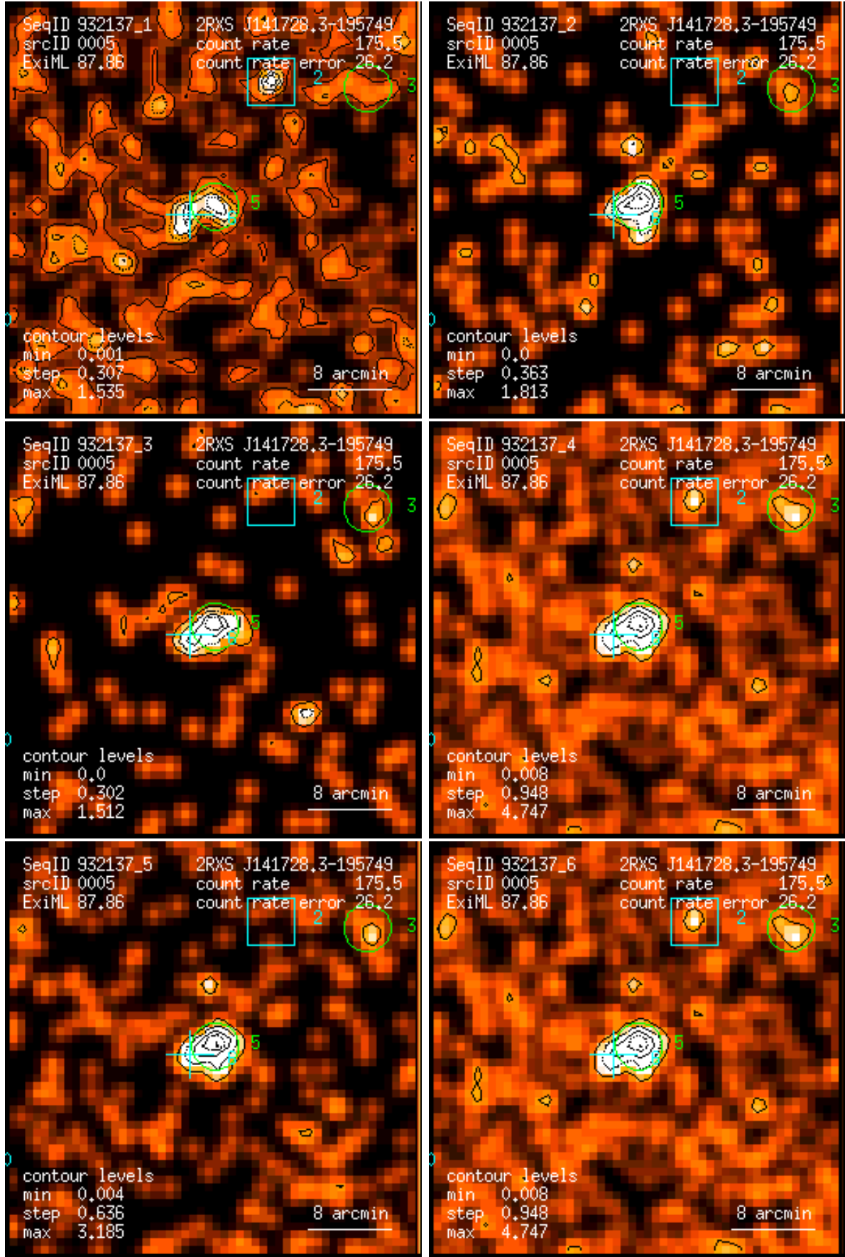
Figure 5: RASS 932137: detection 0005: band rate images, Gaussian filter: (1) PSPC channels 11 – 41, (2) 52 – 90, (3) 91 – 201, (4) 11 – 235, (5) 52 – 201, (6) 11 – 201. Broad band rates in counts/ks. Band rate contour levels in counts/ks/arcmin 2 .
