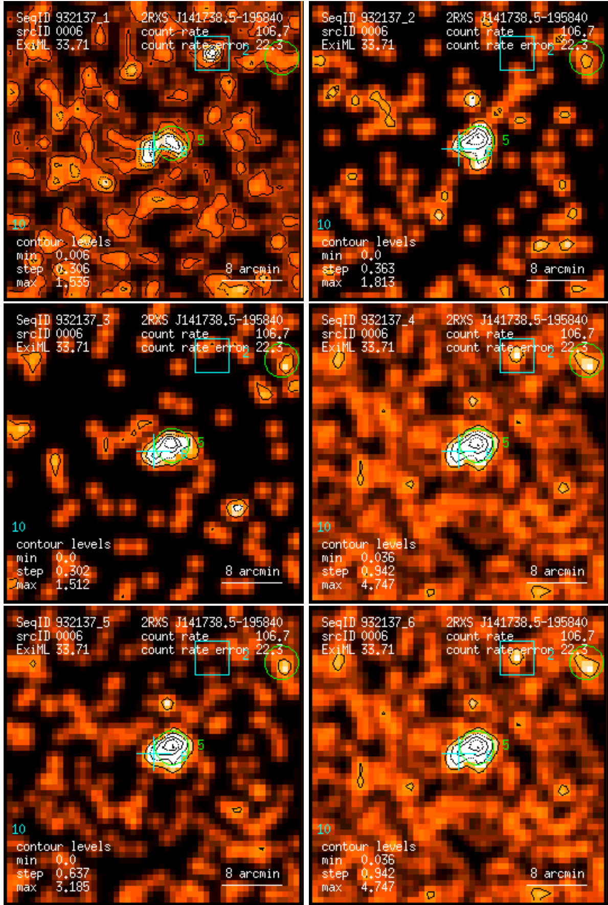
Figure 6: RASS 932137: detection 0006: band rate images, Gaussian filter: (1) PSPC channels 11 – 41, (2) 52 – 90, (3) 91 – 201, (4) 11 – 235, (5) 52 – 201, (6) 11 – 201. Broad band rates in counts/ks. Band rate contour levels in counts/ks/arcmin 2 .
