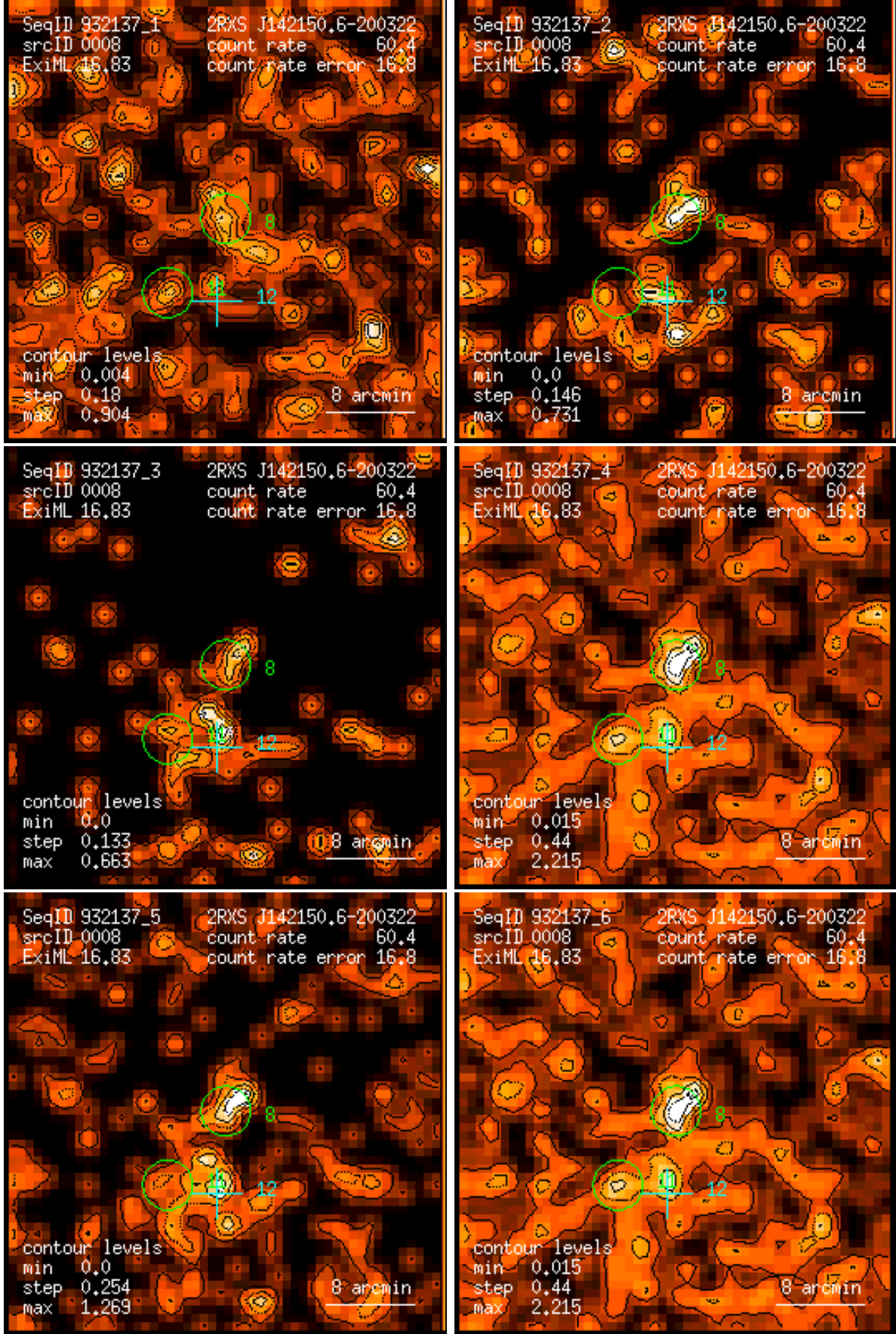
Figure 8: RASS 932137: detection 0008: band rate images, Gaussian filter: (1) PSPC channels 11 – 41, (2) 52 – 90, (3) 91 – 201, (4) 11 – 235, (5) 52 – 201, (6) 11 – 201. Broad band rates in counts/ks. Band rate contour levels in counts/ks/arcmin 2 .
