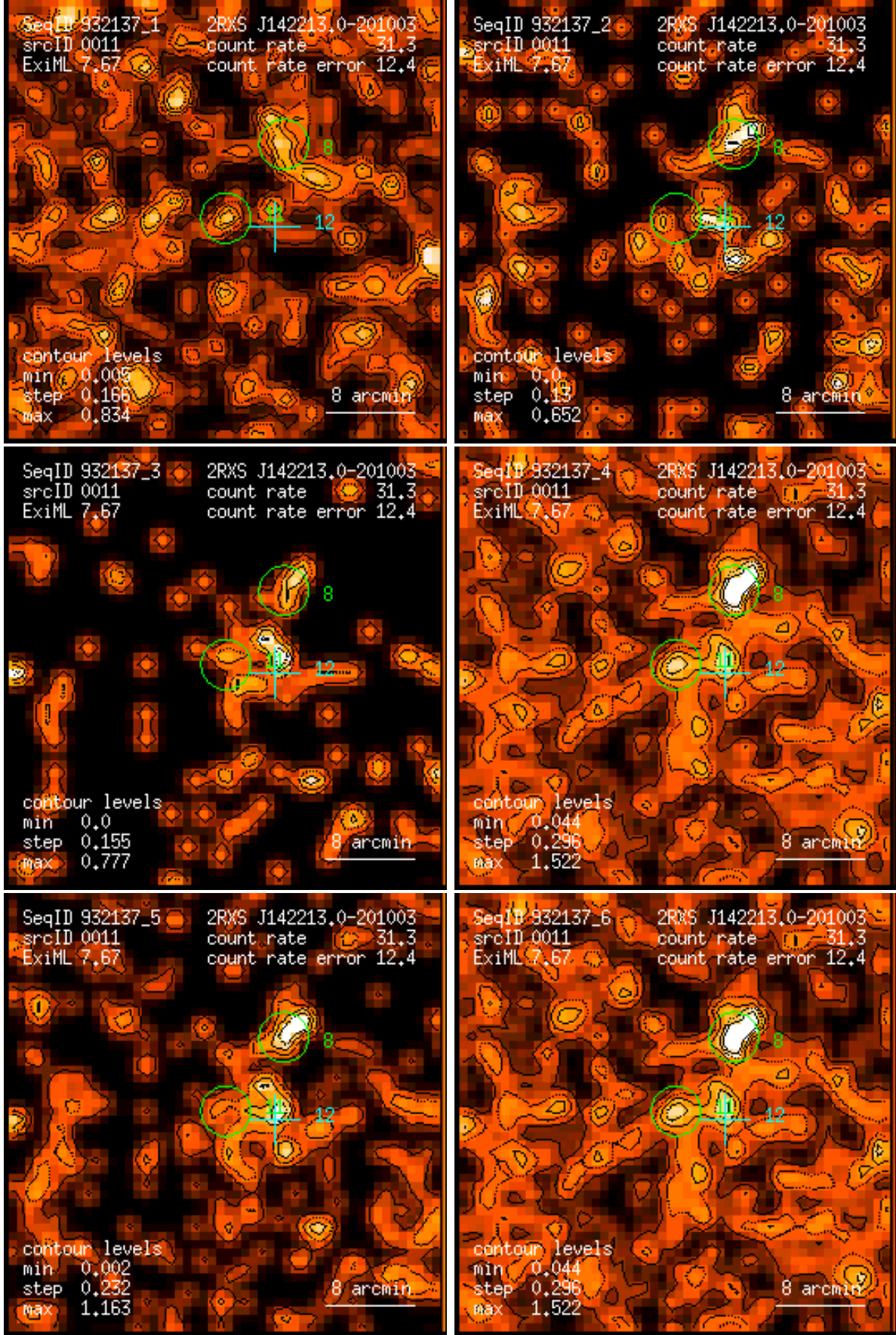
Figure 11: RASS 932137: detection 0011: band rate images, Gaussian filter: (1) PSPC channels 11 – 41, (2) 52 – 90, (3) 91 – 201, (4) 11 – 235, (5) 52 – 201, (6) 11 – 201. Broad band rates in counts/ks. Band rate contour levels in counts/ks/arcmin 2 .
