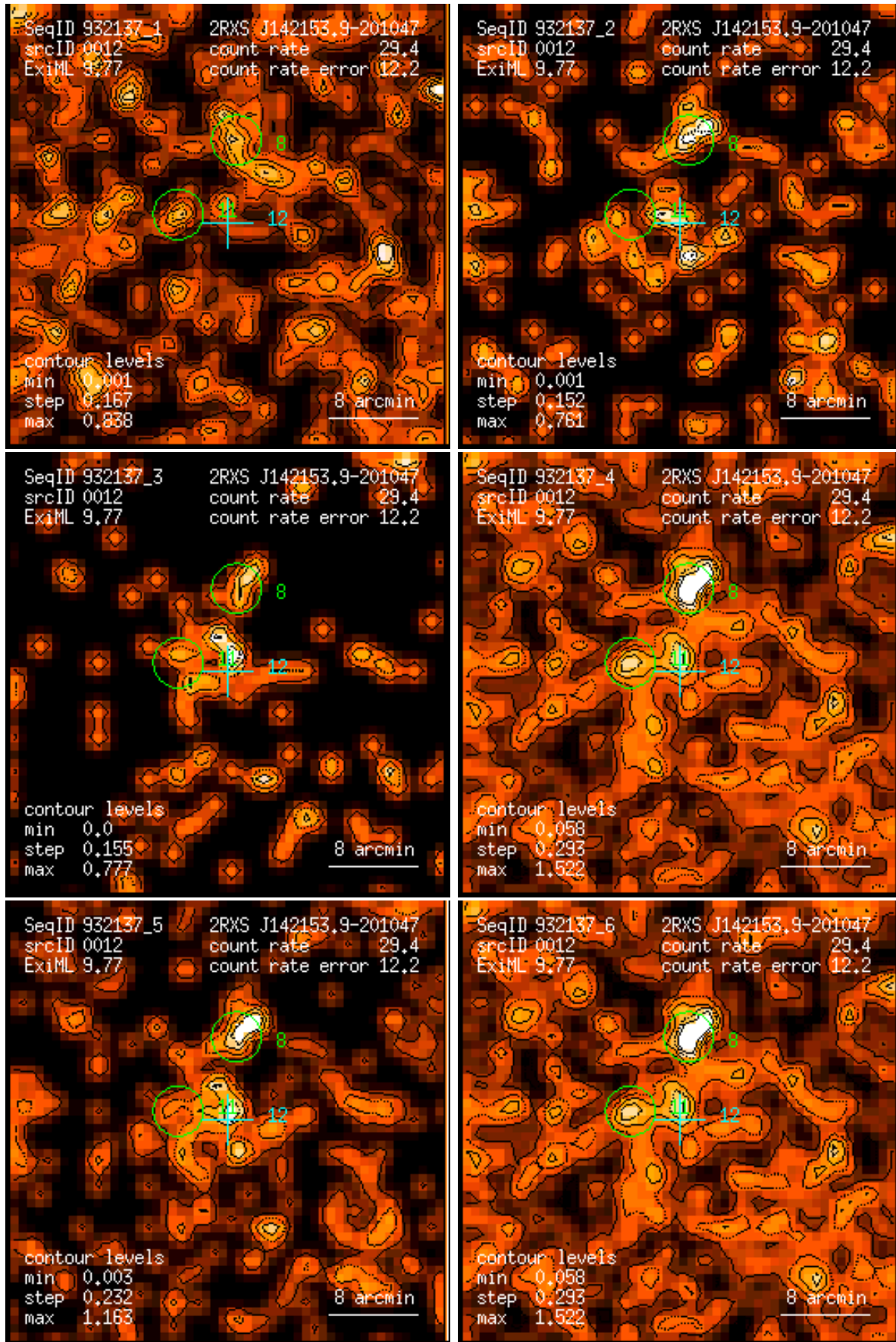
Figure 12: RASS 932137: detection 0012: band rate images, Gaussian filter: (1) PSPC channels 11 – 41, (2) 52 – 90, (3) 91 – 201, (4) 11 – 235, (5) 52 – 201, (6) 11 – 201. Broad band rates in counts/ks. Band rate contour levels in counts/ks/arcmin 2 .
