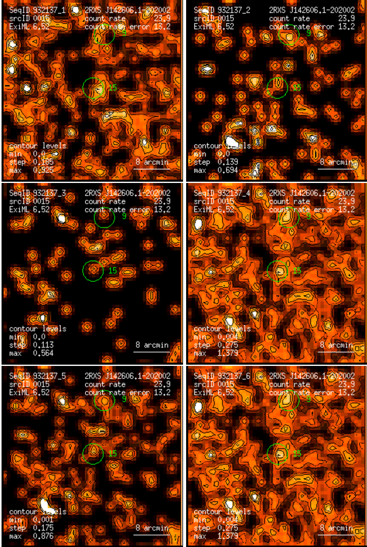
Figure 15: RASS 932137: detection 0015: band rate images, Gaussian filter: (1) PSPC channels 11 – 41, (2) 52 – 90, (3) 91 – 201, (4) 11 – 235, (5) 52 – 201, (6) 11 – 201. Broad band rates in counts/ks. Band rate contour levels in counts/ks/arcmin 2 .
