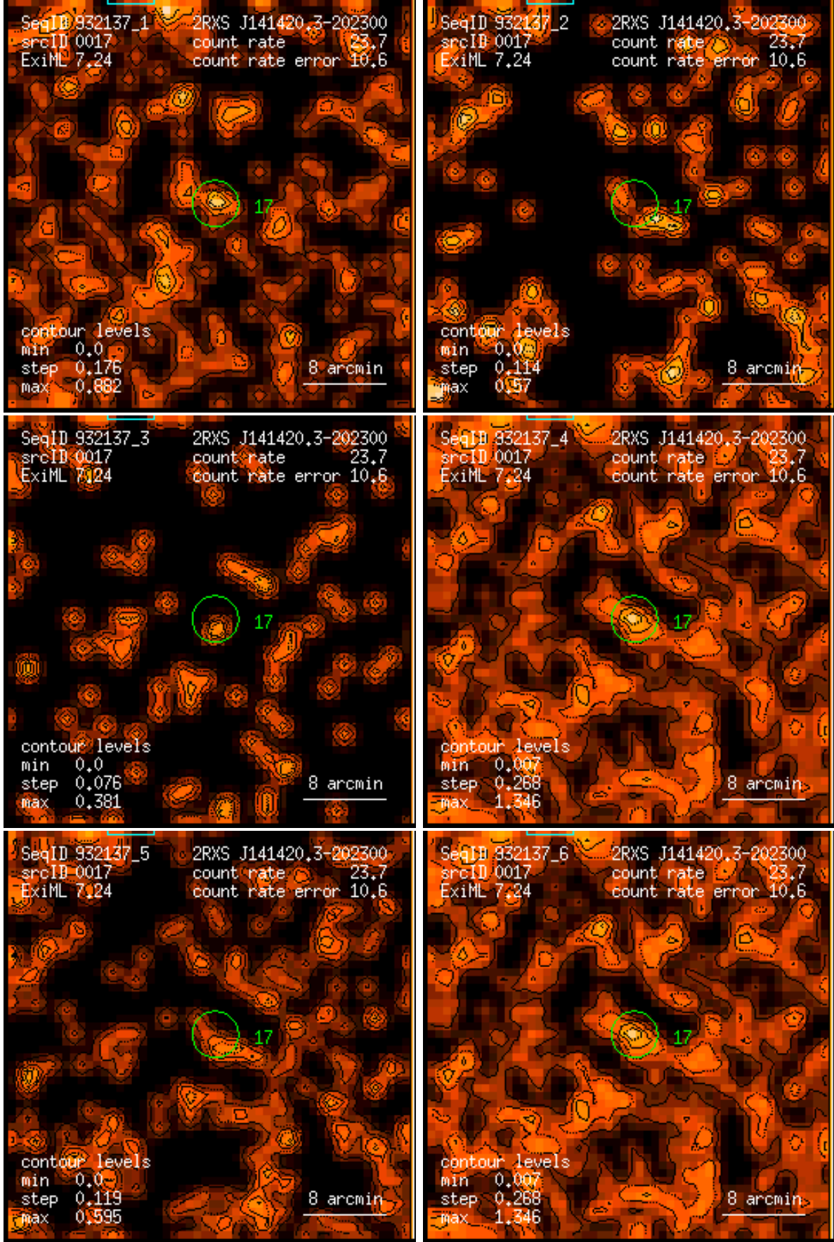
Figure 17: RASS 932137: detection 0017: band rate images, Gaussian filter: (1) PSPC channels 11 – 41, (2) 52 – 90, (3) 91 – 201, (4) 11 – 235, (5) 52 – 201, (6) 11 – 201. Broad band rates in counts/ks. Band rate contour levels in counts/ks/arcmin 2 .
