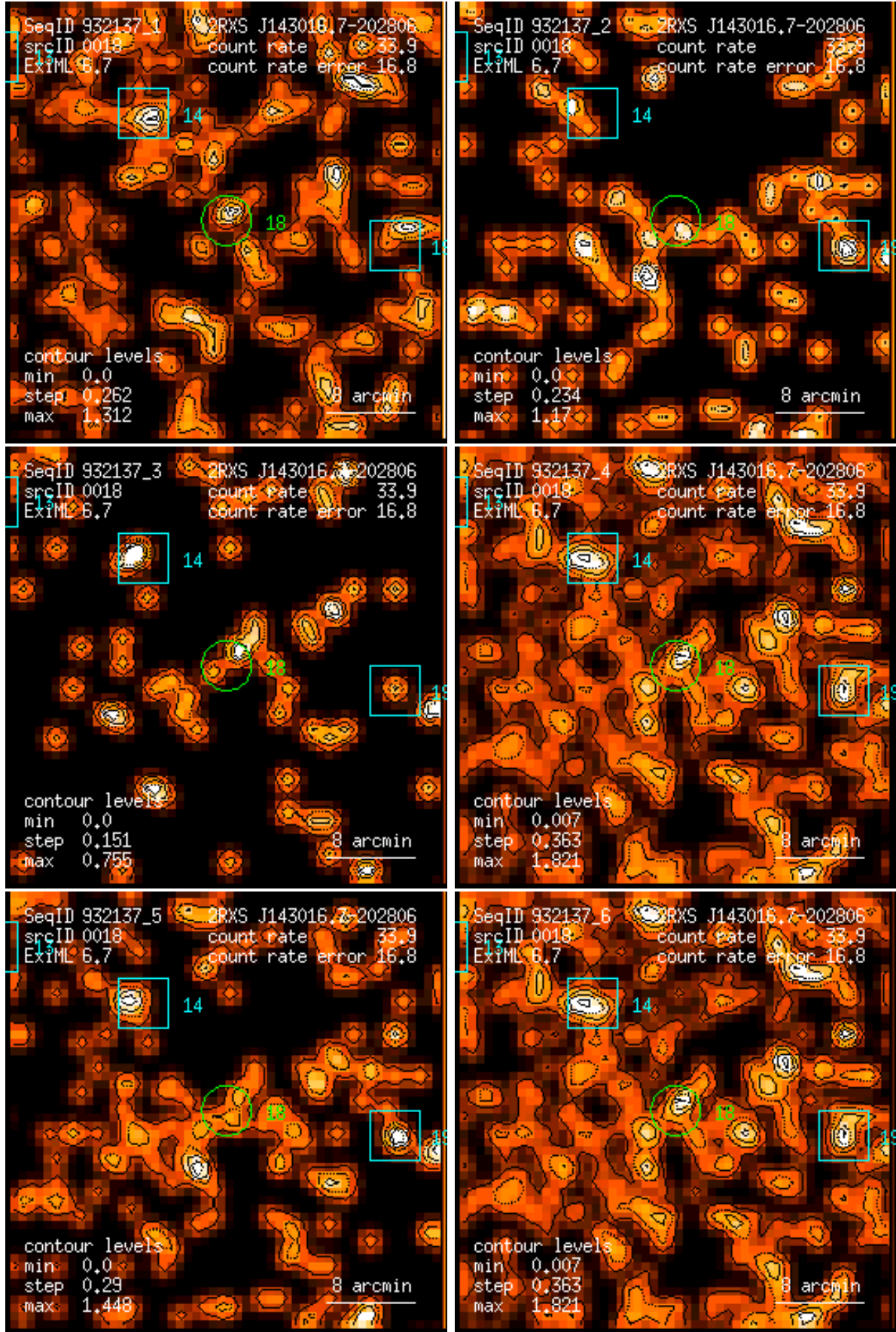
Figure 18: RASS 932137: detection 0018: band rate images, Gaussian filter: (1) PSPC channels 11 – 41, (2) 52 – 90, (3) 91 – 201, (4) 11 – 235, (5) 52 – 201, (6) 11 – 201. Broad band rates in counts/ks. Band rate contour levels in counts/ks/arcmin 2 .
