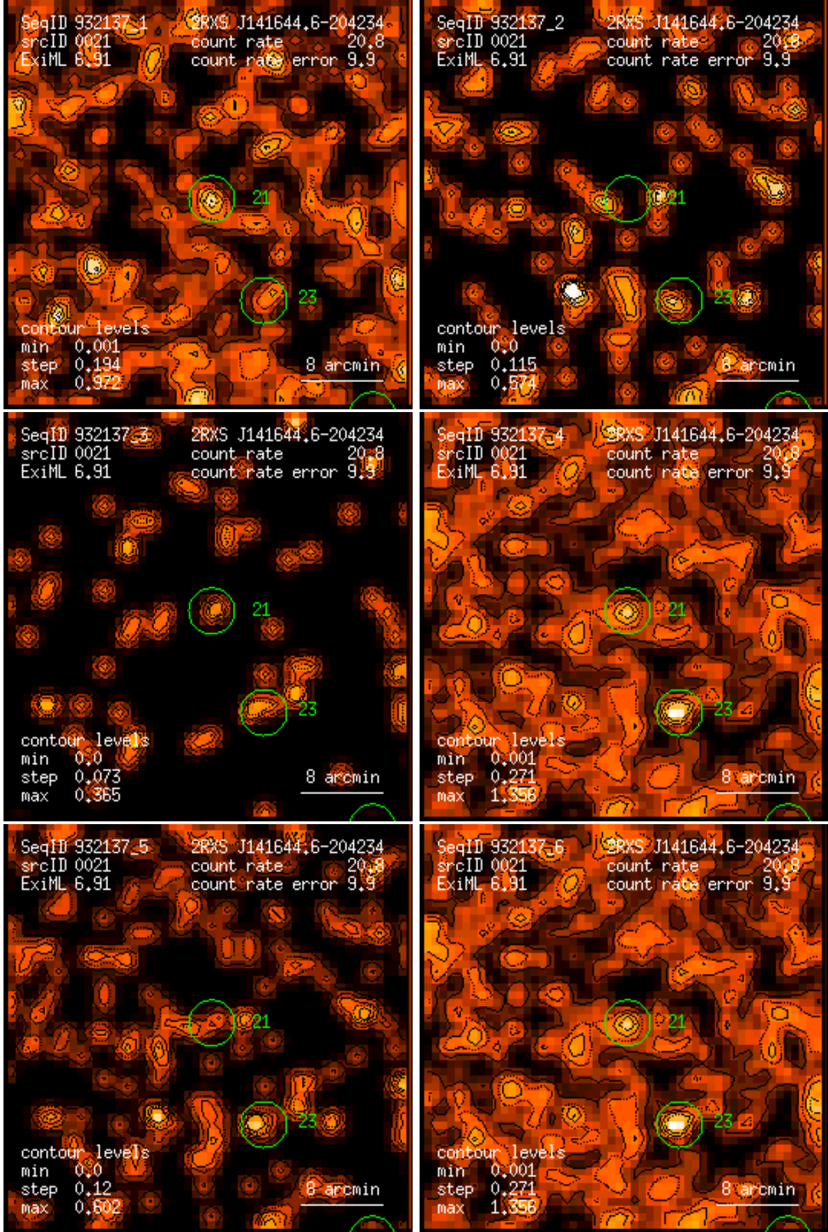
Figure 21: RASS 932137: detection 0021: band rate images, Gaussian filter: (1) PSPC channels 11 – 41, (2) 52 – 90, (3) 91 – 201, (4) 11 – 235, (5) 52 – 201, (6) 11 – 201. Broad band rates in counts/ks. Band rate contour levels in counts/ks/arcmin 2 .
