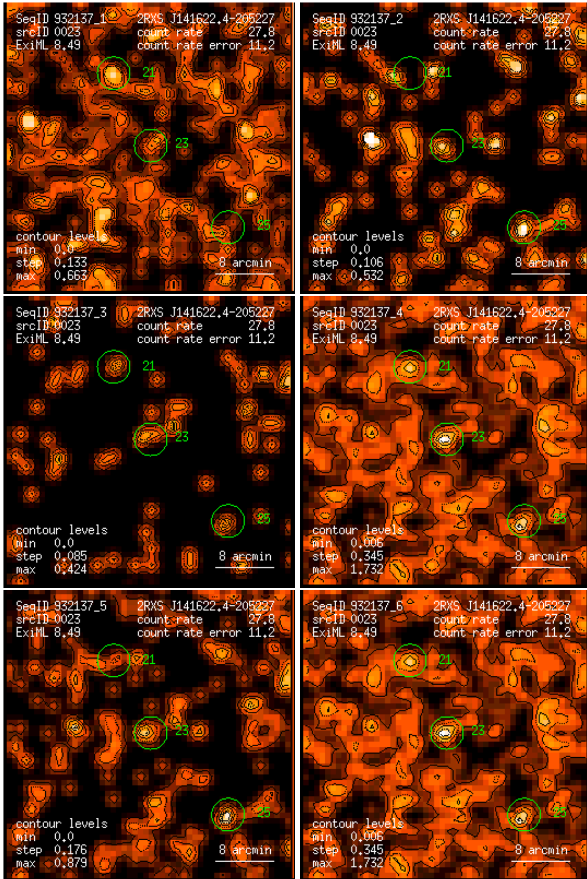
Figure 23: RASS 932137: detection 0023: band rate images, Gaussian filter: (1) PSPC channels 11 – 41, (2) 52 – 90, (3) 91 – 201, (4) 11 – 235, (5) 52 – 201, (6) 11 – 201. Broad band rates in counts/ks. Band rate contour levels in counts/ks/arcmin 2 .
