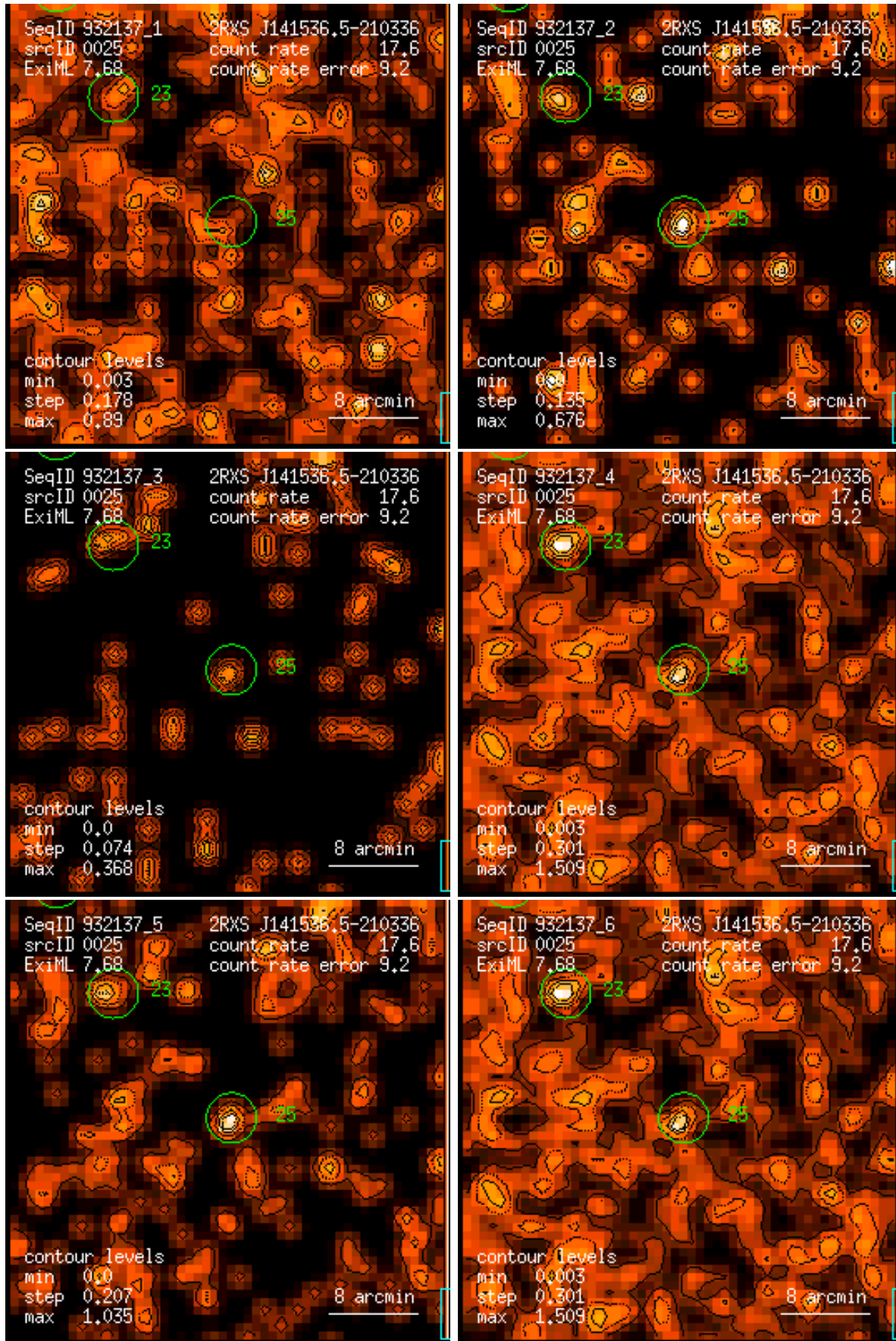
Figure 25: RASS 932137: detection 0025: band rate images, Gaussian filter: (1) PSPC channels 11 – 41, (2) 52 – 90, (3) 91 – 201, (4) 11 – 235, (5) 52 – 201, (6) 11 – 201. Broad band rates in counts/ks. Band rate contour levels in counts/ks/arcmin 2 .
