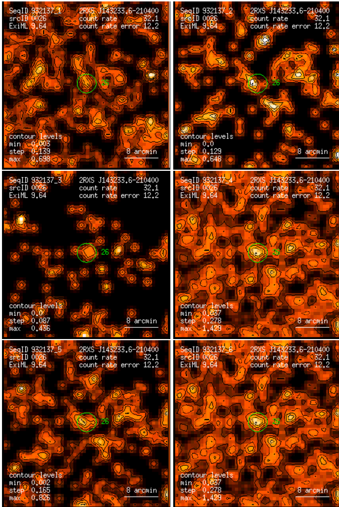
Figure 26: RASS 932137: detection 0026: band rate images, Gaussian filter: (1) PSPC channels 11 – 41, (2) 52 – 90, (3) 91 – 201, (4) 11 – 235, (5) 52 – 201, (6) 11 – 201. Broad band rates in counts/ks. Band rate contour levels in counts/ks/arcmin 2 .
