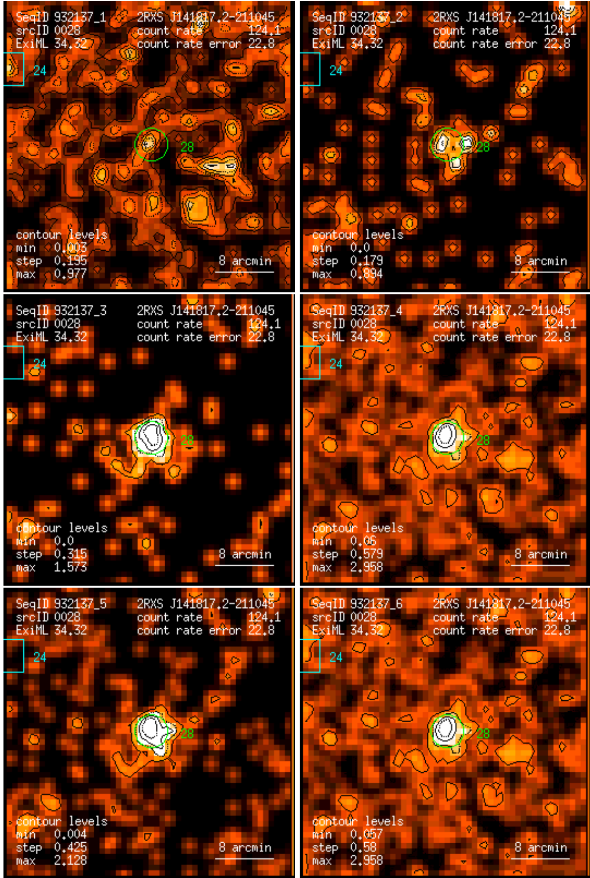
Figure 28: RASS 932137: detection 0028: band rate images, Gaussian filter: (1) PSPC channels 11 – 41, (2) 52 – 90, (3) 91 – 201, (4) 11 – 235, (5) 52 – 201, (6) 11 – 201. Broad band rates in counts/ks. Band rate contour levels in counts/ks/arcmin 2 .
