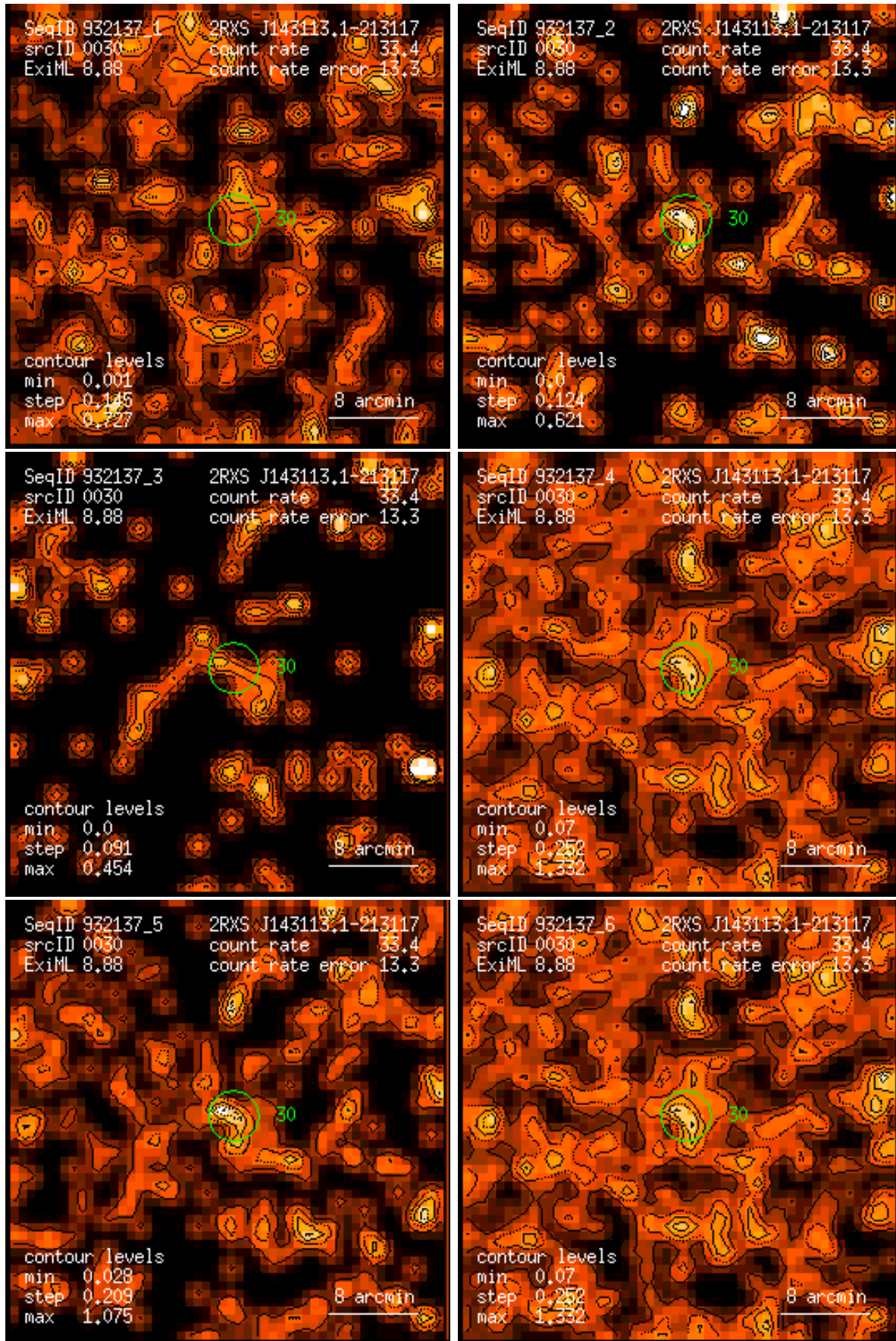
Figure 30: RASS 932137: detection 0030: band rate images, Gaussian filter: (1) PSPC channels 11 – 41, (2) 52 – 90, (3) 91 – 201, (4) 11 – 235, (5) 52 – 201, (6) 11 – 201. Broad band rates in counts/ks. Band rate contour levels in counts/ks/arcmin 2 .
