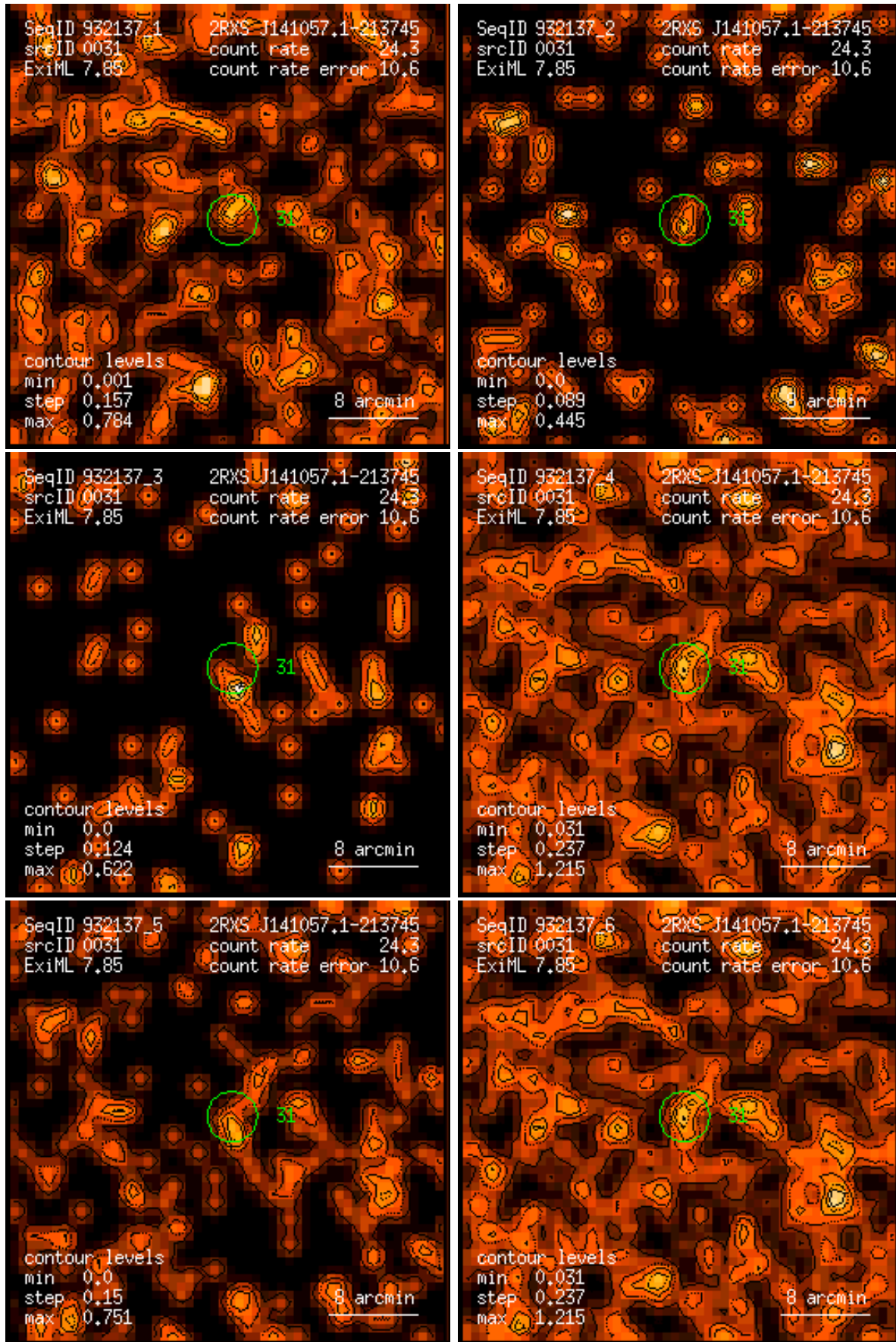
Figure 31: RASS 932137: detection 0031: band rate images, Gaussian filter: (1) PSPC channels 11 – 41, (2) 52 – 90, (3) 91 – 201, (4) 11 – 235, (5) 52 – 201, (6) 11 – 201. Broad band rates in counts/ks. Band rate contour levels in counts/ks/arcmin 2 .
