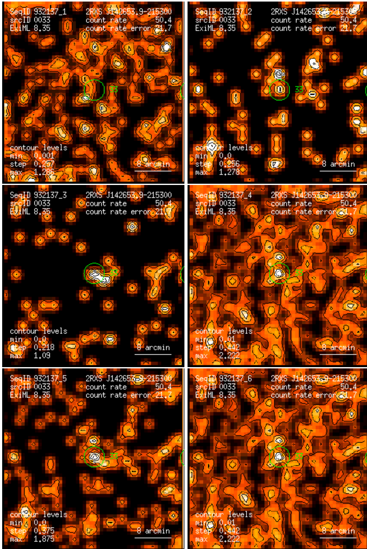
Figure 33: RASS 932137: detection 0033: band rate images, Gaussian filter: (1) PSPC channels 11 – 41, (2) 52 – 90, (3) 91 – 201, (4) 11 – 235, (5) 52 – 201, (6) 11 – 201. Broad band rates in counts/ks. Band rate contour levels in counts/ks/arcmin 2 .
