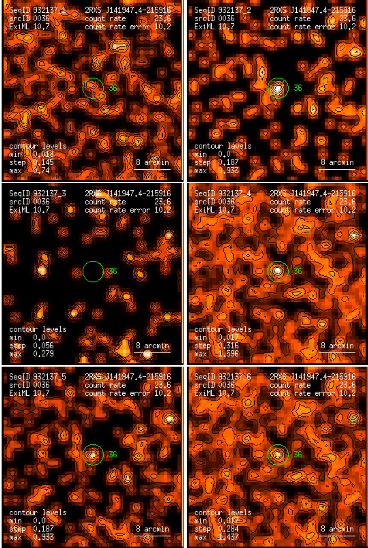
Figure 36: RASS 932137: detection 0036: band rate images, Gaussian filter: (1) PSPC channels 11 – 41, (2) 52 – 90, (3) 91 – 201, (4) 11 – 235, (5) 52 – 201, (6) 11 – 201. Broad band rates in counts/ks. Band rate contour levels in counts/ks/arcmin 2 .
