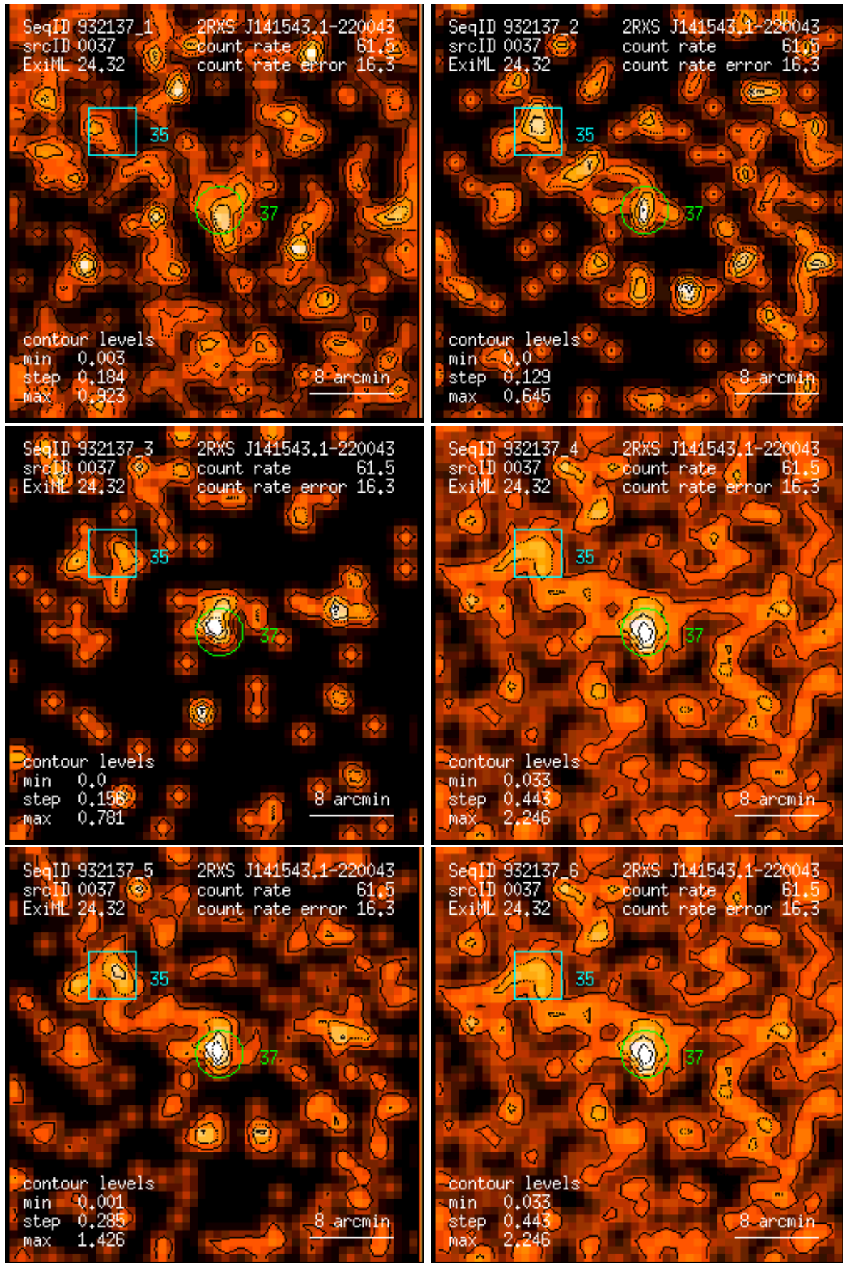
Figure 37: RASS 932137: detection 0037: band rate images, Gaussian filter: (1) PSPC channels 11 – 41, (2) 52 – 90, (3) 91 – 201, (4) 11 – 235, (5) 52 – 201, (6) 11 – 201. Broad band rates in counts/ks. Band rate contour levels in counts/ks/arcmin 2 .
