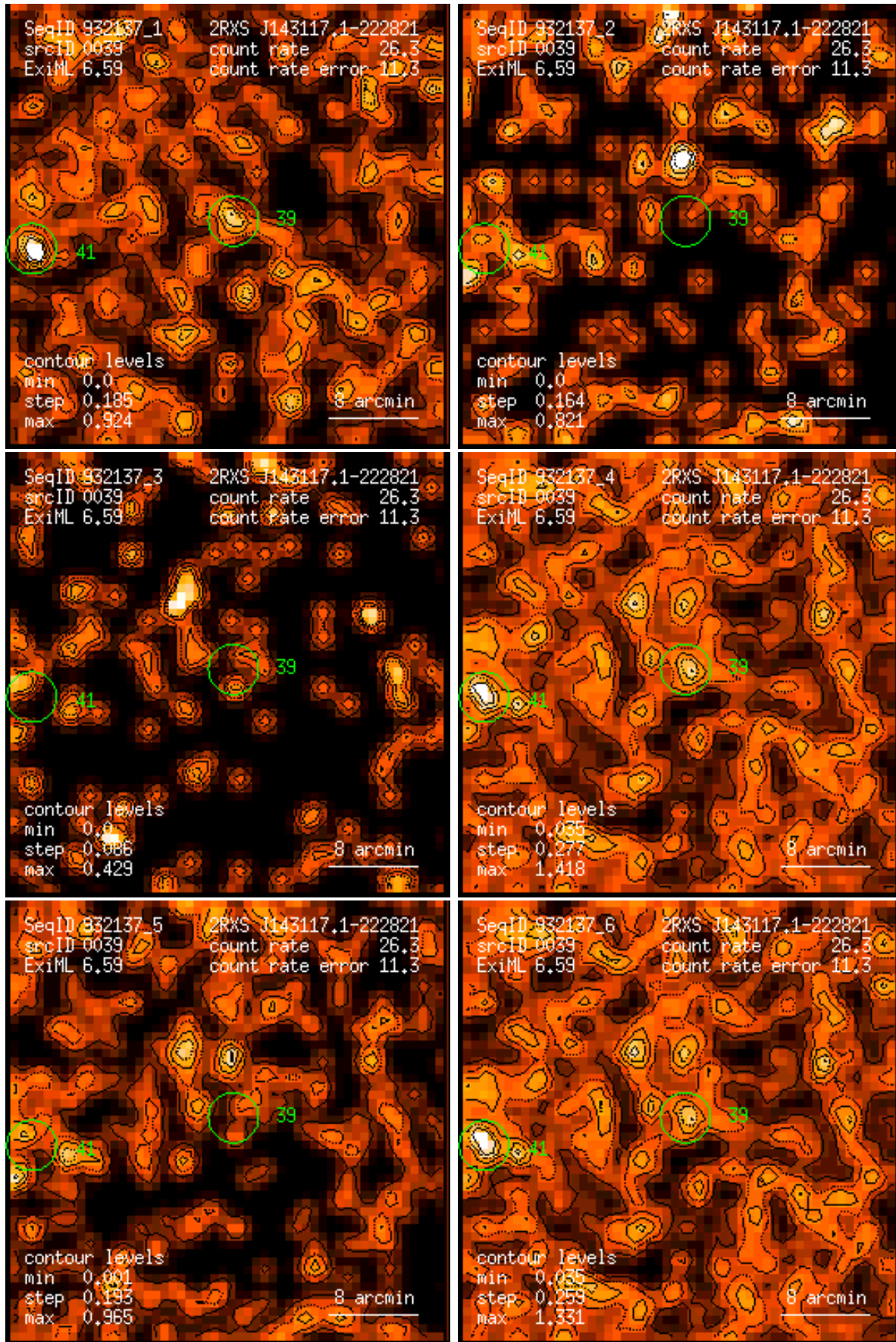
Figure 39: RASS 932137: detection 0039: band rate images, Gaussian filter: (1) PSPC channels 11 – 41, (2) 52 – 90, (3) 91 – 201, (4) 11 – 235, (5) 52 – 201, (6) 11 – 201. Broad band rates in counts/ks. Band rate contour levels in counts/ks/arcmin 2 .
