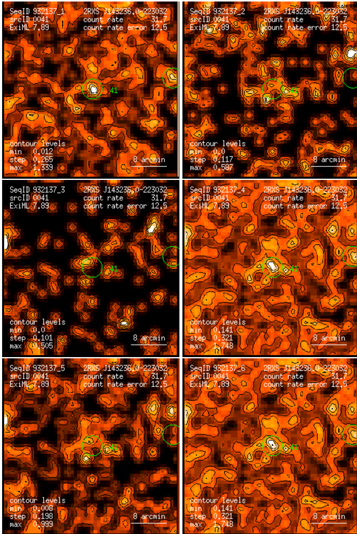
Figure 41: RASS 932137: detection 0041: band rate images, Gaussian filter: (1) PSPC channels 11 – 41, (2) 52 – 90, (3) 91 – 201, (4) 11 – 235, (5) 52 – 201, (6) 11 – 201. Broad band rates in counts/ks. Band rate contour levels in counts/ks/arcmin 2 .
