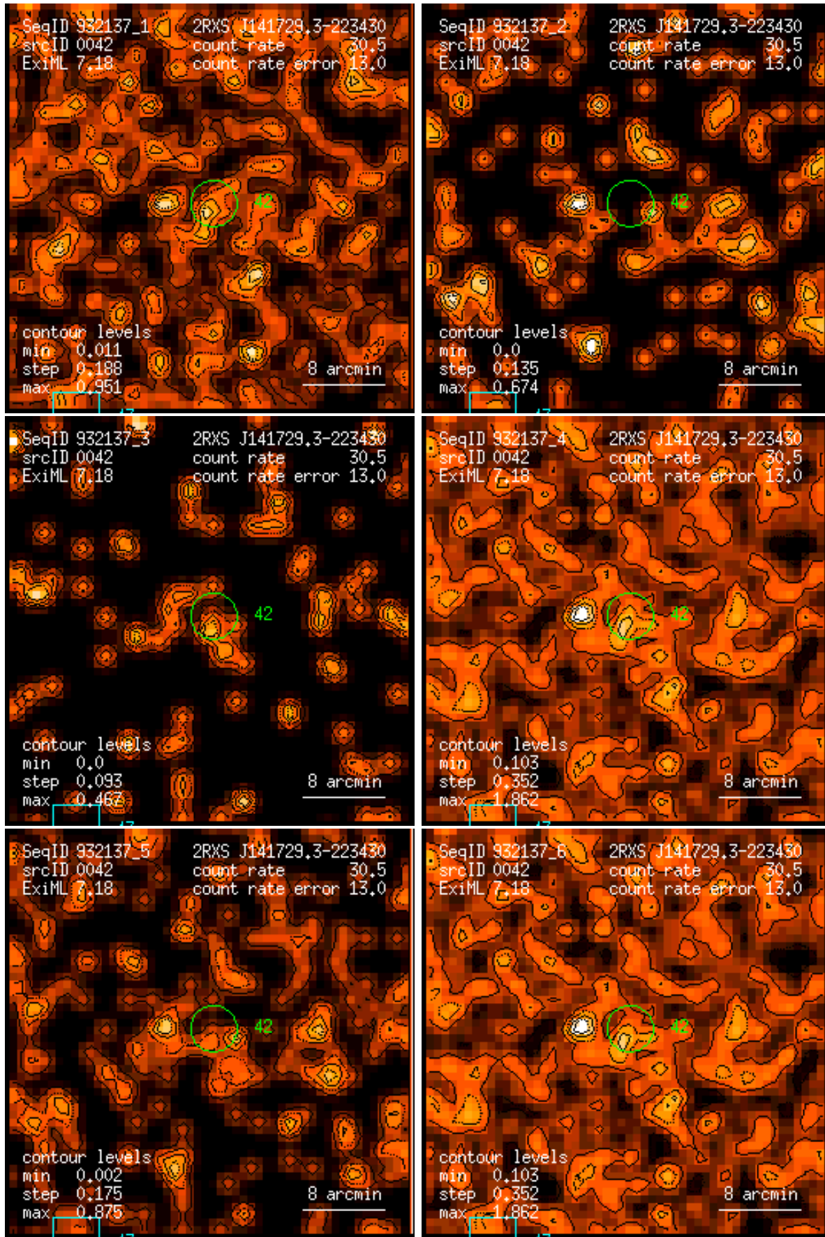
Figure 42: RASS 932137: detection 0042: band rate images, Gaussian filter: (1) PSPC channels 11 – 41, (2) 52 – 90, (3) 91 – 201, (4) 11 – 235, (5) 52 – 201, (6) 11 – 201. Broad band rates in counts/ks. Band rate contour levels in counts/ks/arcmin 2 .
