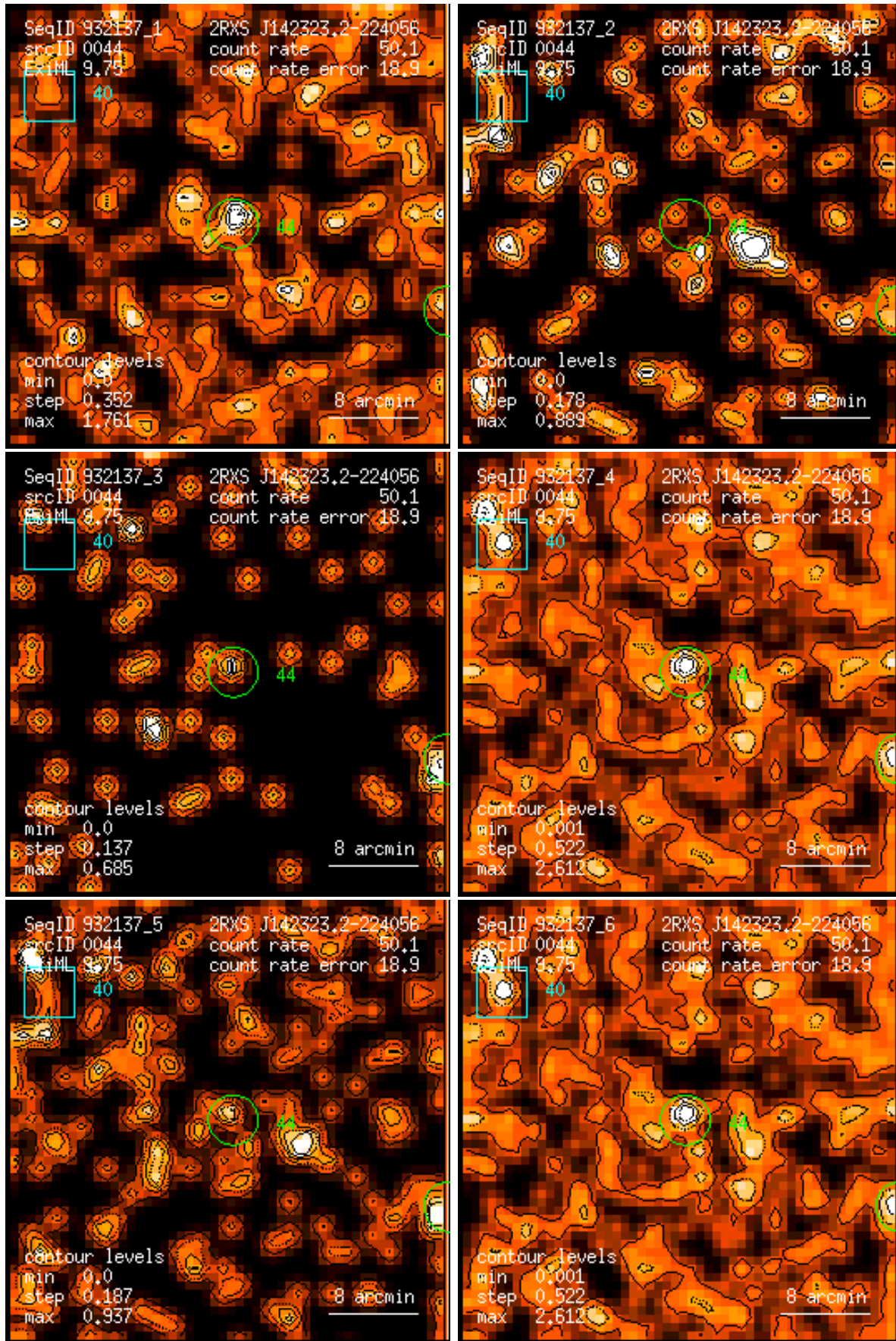
Figure 44: RASS 932137: detection 0044: band rate images, Gaussian filter: (1) PSPC channels 11 – 41, (2) 52 – 90, (3) 91 – 201, (4) 11 – 235, (5) 52 – 201, (6) 11 – 201. Broad band rates in counts/ks. Band rate contour levels in counts/ks/arcmin 2 .
