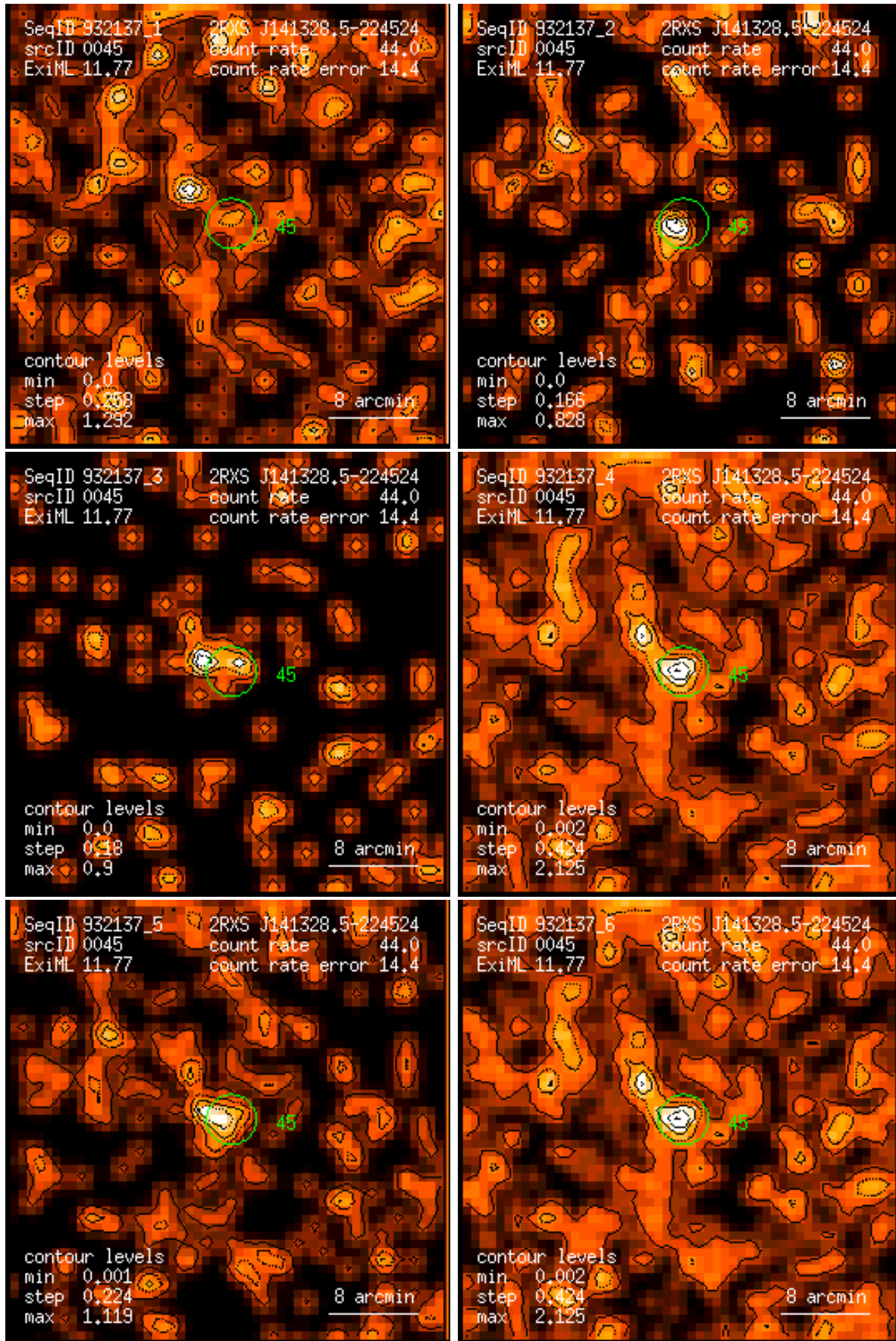
Figure 45: RASS 932137: detection 0045: band rate images, Gaussian filter: (1) PSPC channels 11 – 41, (2) 52 – 90, (3) 91 – 201, (4) 11 – 235, (5) 52 – 201, (6) 11 – 201. Broad band rates in counts/ks. Band rate contour levels in counts/ks/arcmin 2 .
