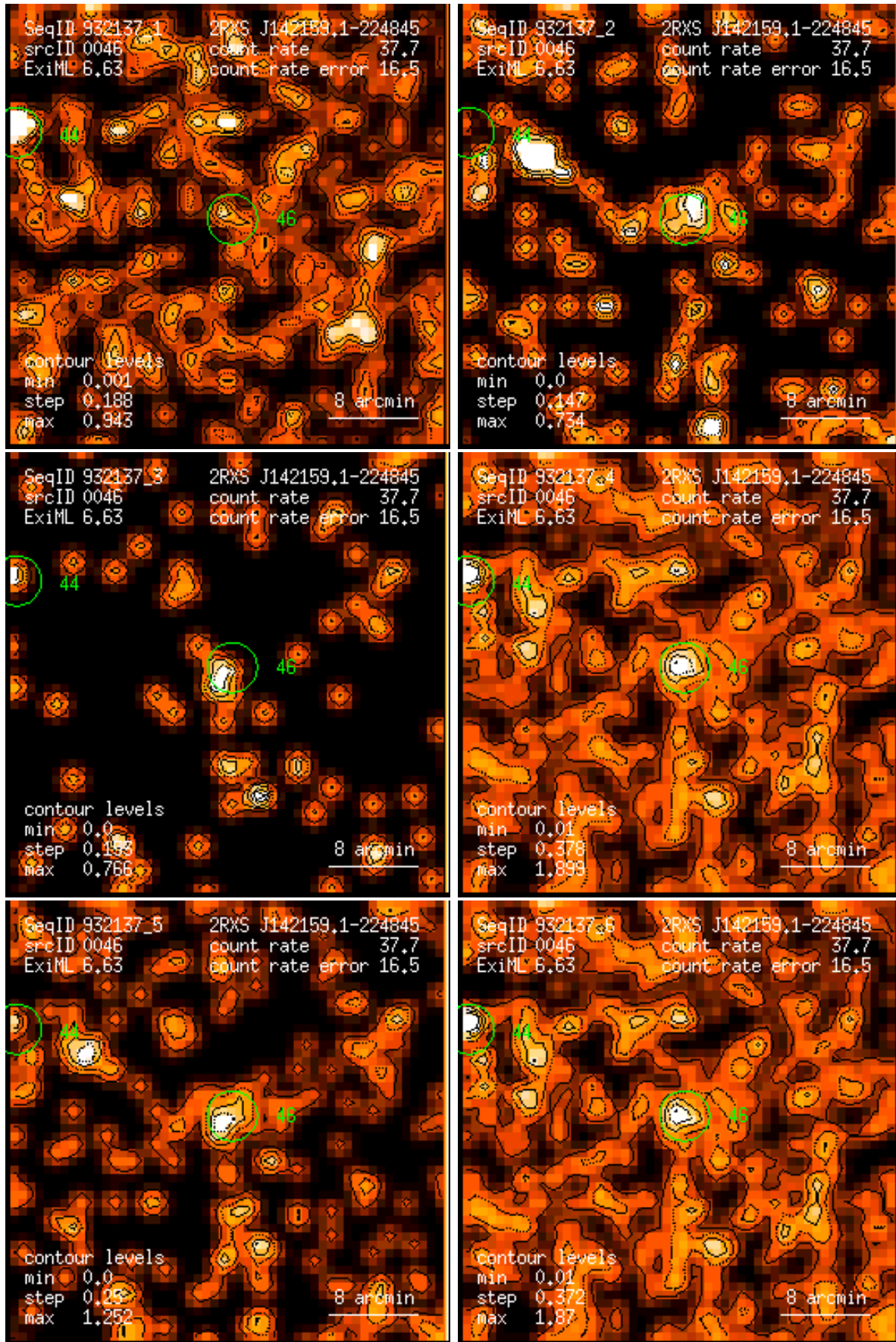
Figure 46: RASS 932137: detection 0046: band rate images, Gaussian filter: (1) PSPC channels 11 – 41, (2) 52 – 90, (3) 91 – 201, (4) 11 – 235, (5) 52 – 201, (6) 11 – 201. Broad band rates in counts/ks. Band rate contour levels in counts/ks/arcmin 2 .
