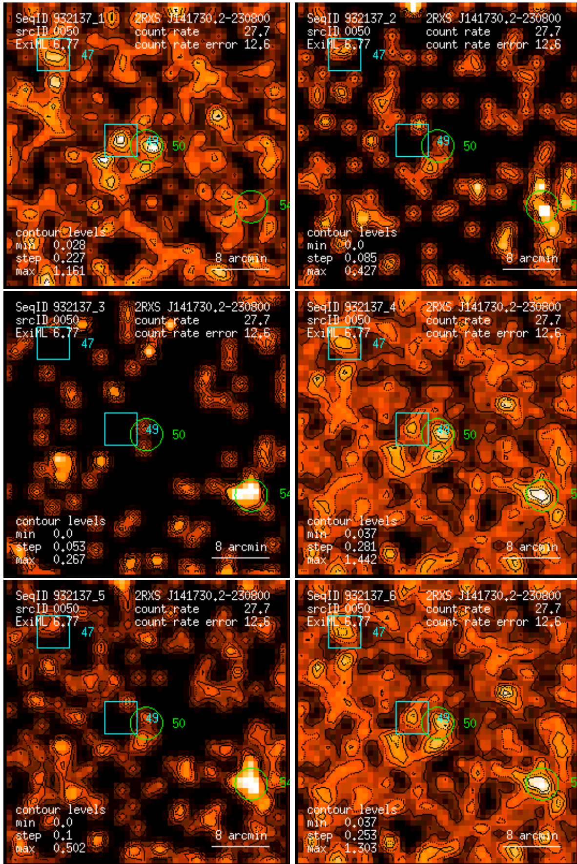
Figure 50: RASS 932137: detection 0050: band rate images, Gaussian filter: (1) PSPC channels 11 – 41, (2) 52 – 90, (3) 91 – 201, (4) 11 – 235, (5) 52 – 201, (6) 11 – 201. Broad band rates in counts/ks. Band rate contour levels in counts/ks/arcmin 2 .
