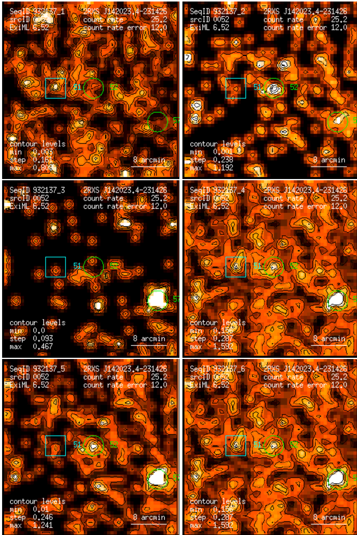
Figure 52: RASS 932137: detection 0052: band rate images, Gaussian filter: (1) PSPC channels 11 – 41, (2) 52 – 90, (3) 91 – 201, (4) 11 – 235, (5) 52 – 201, (6) 11 – 201. Broad band rates in counts/ks. Band rate contour levels in counts/ks/arcmin 2 .
