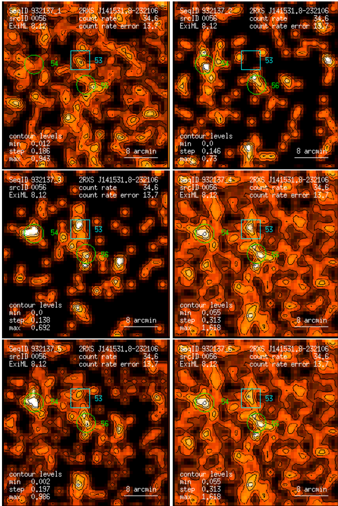
Figure 56: RASS 932137: detection 0056: band rate images, Gaussian filter: (1) PSPC channels 11 – 41, (2) 52 – 90, (3) 91 – 201, (4) 11 – 235, (5) 52 – 201, (6) 11 – 201. Broad band rates in counts/ks. Band rate contour levels in counts/ks/arcmin 2 .
